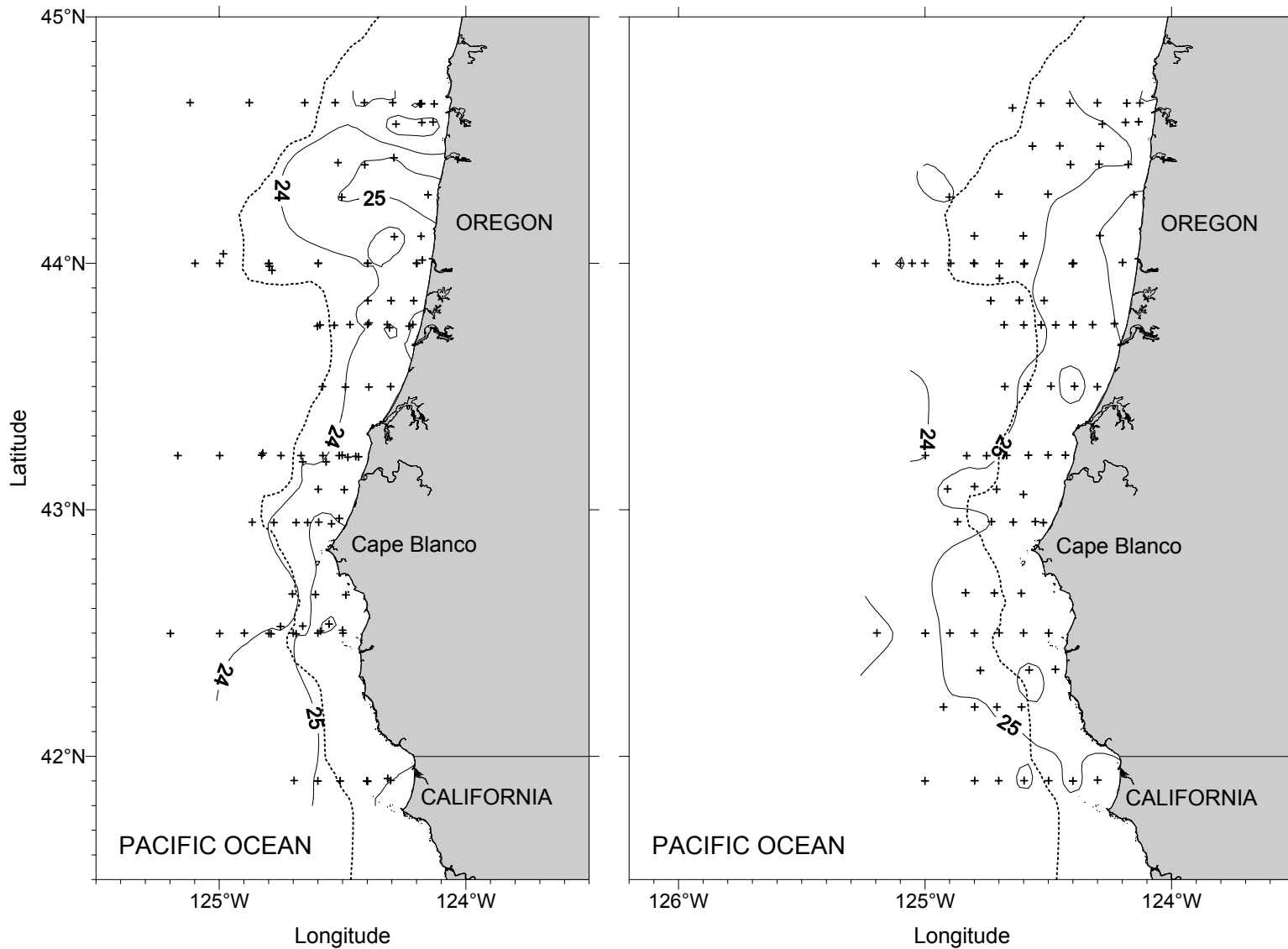
Figure 7. The 1-m depth water density ( \text{kg}/\text{m}^3 ) in June (left) and August (right) 2002. Contour labels are oriented in an uphill direction. Plus signs are locations where measurements were made. The dotted line is the 200-m depth contour.
