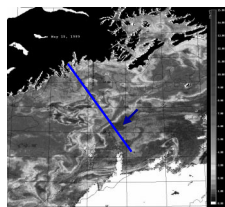
A SeaWiFS false-color image of near-surface chlorophyll pigment concentration on 15 May 1999 shows high chlorophyll concentrations offshore of the shelf-break. (Cloud cover is white).
