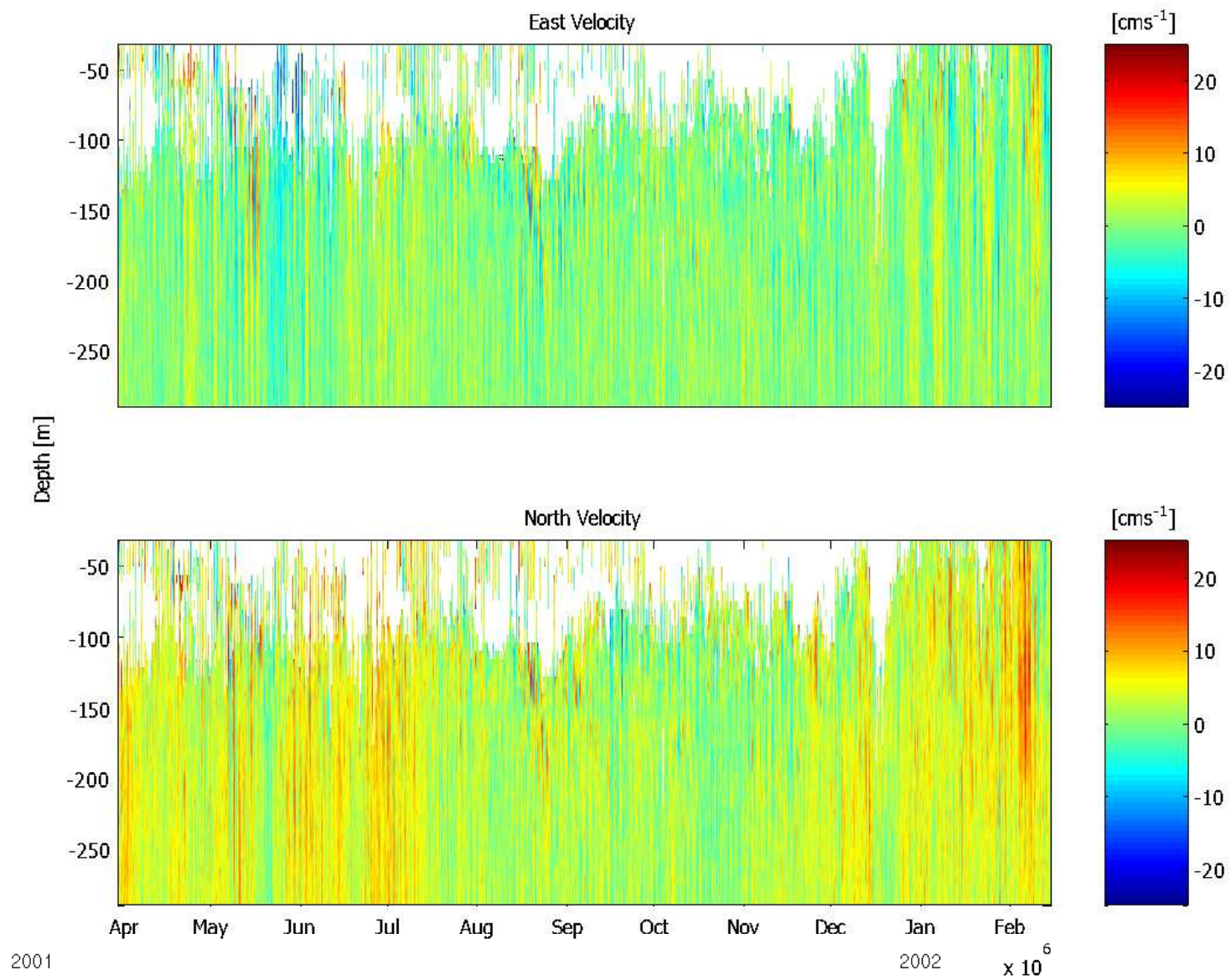
Figure 47: B2: ADCP Velocities
