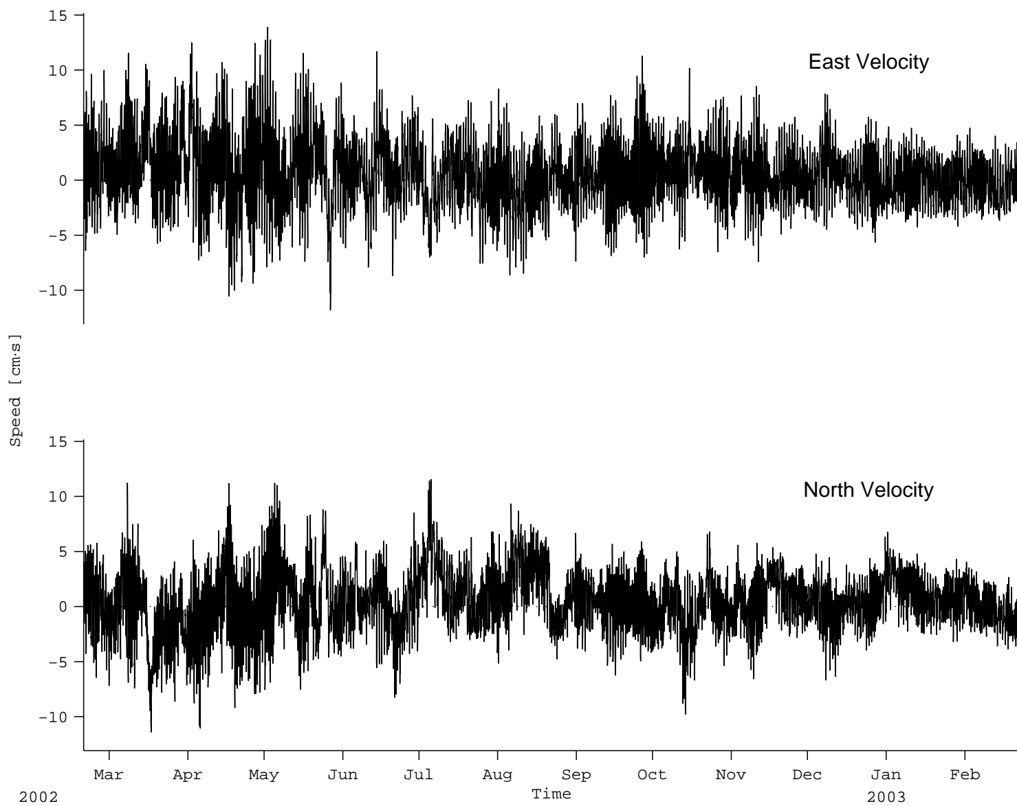
Figure 59: C1: VACM velocity. East Velocity (Top panel), North Velocity (Bottom Panel)
