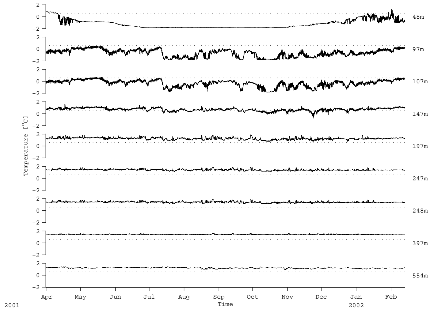
Figure 32: A2: Temperature records
