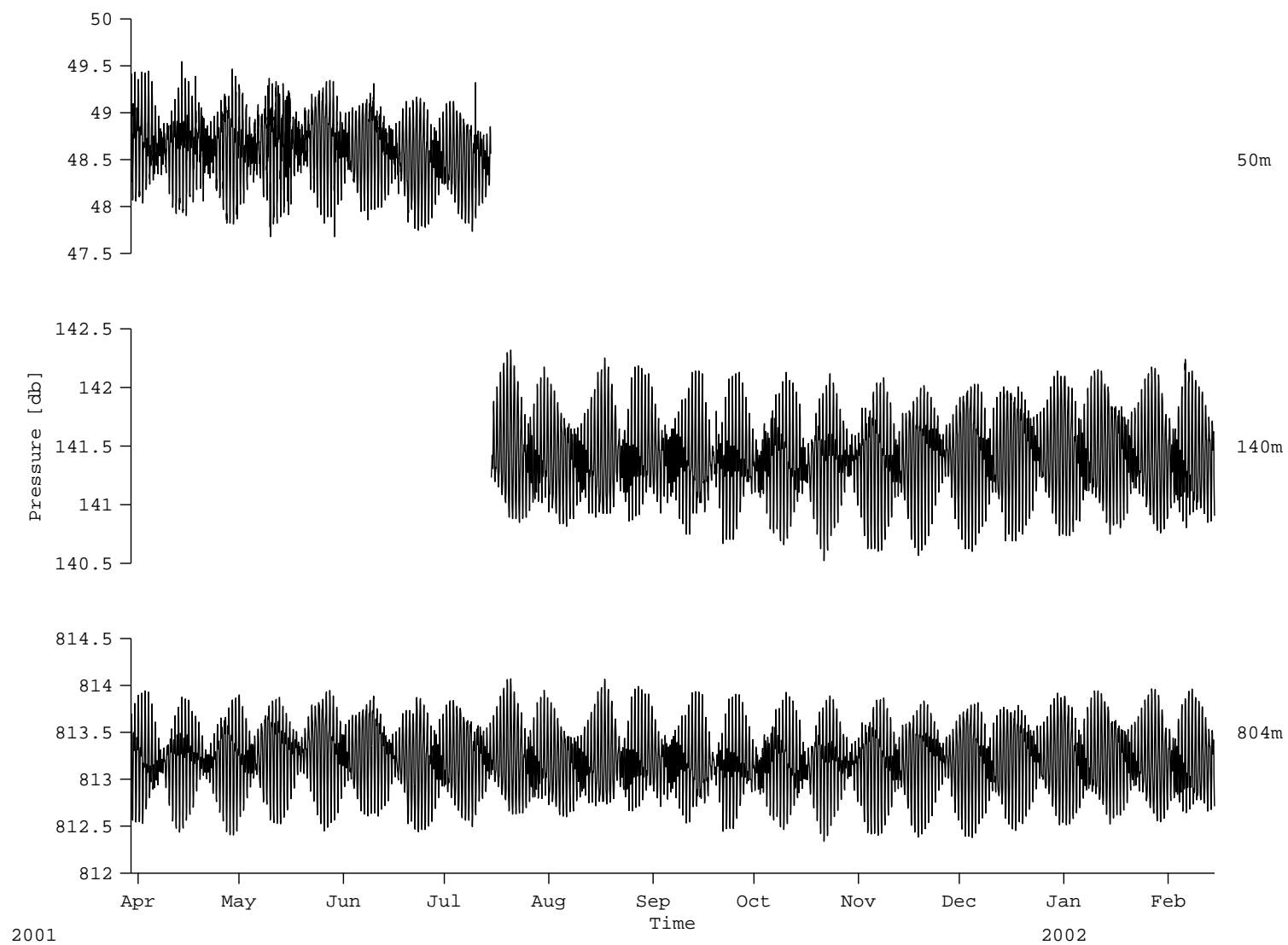
Figure 45: B2: Pressure records
