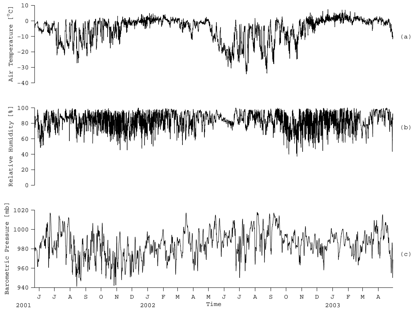
Figure 73: Air temperature (a), relative humidity (b) and barometric pressure (c) measured with the AWS at Dismal Island
