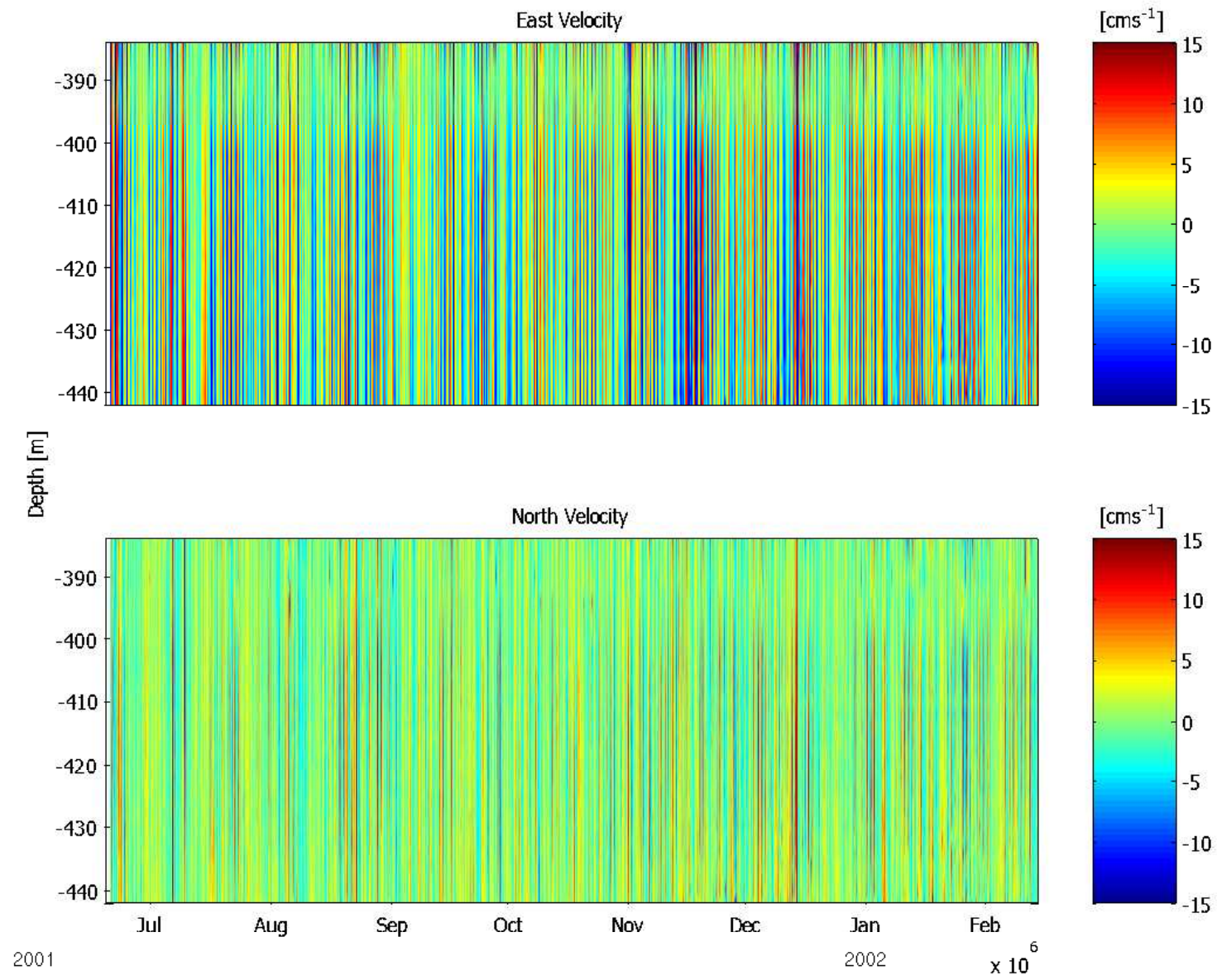
Figure 55: B3: ADCP Velocities, 378m
