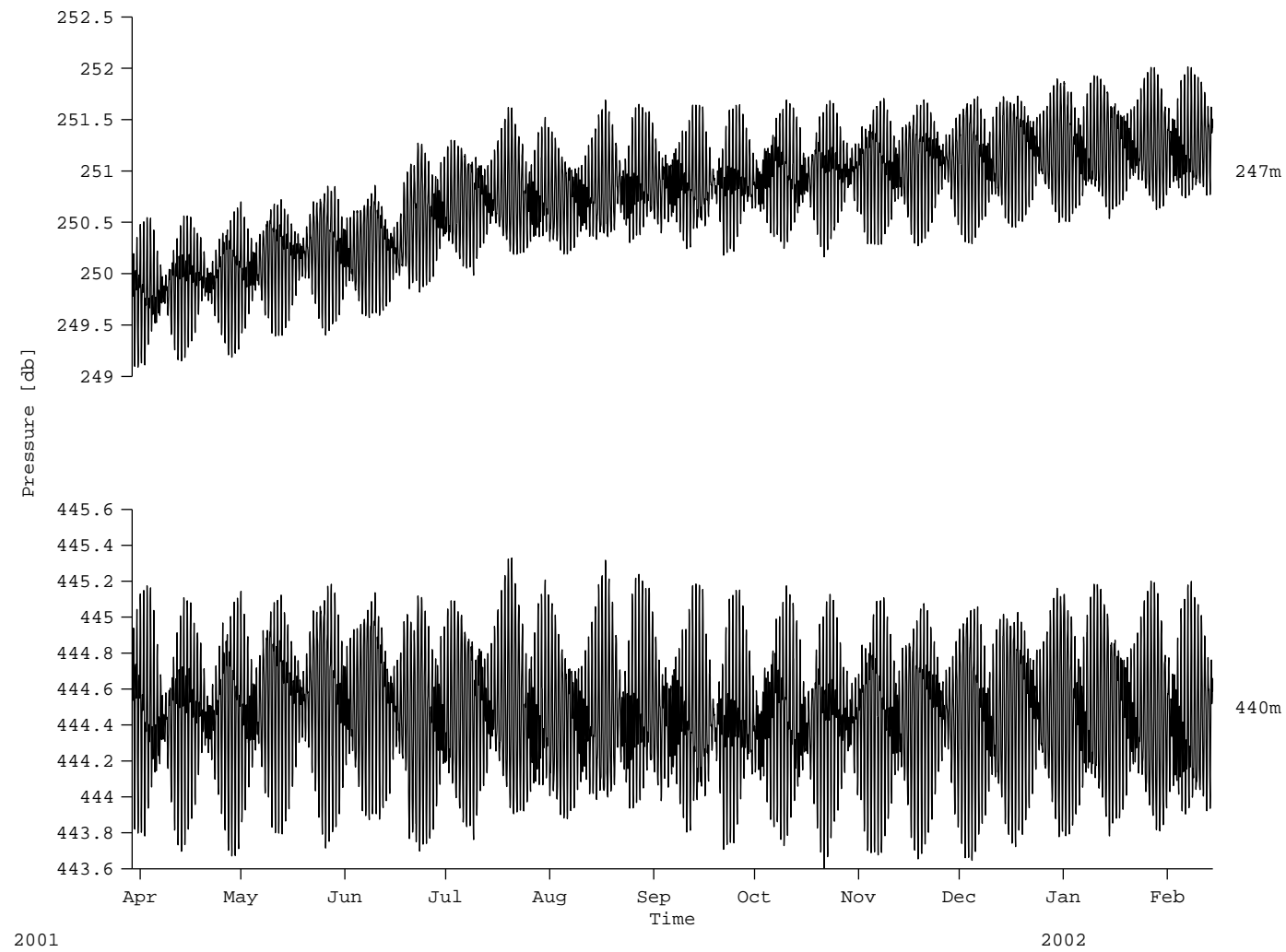
Figure 51: B3: Pressure records
