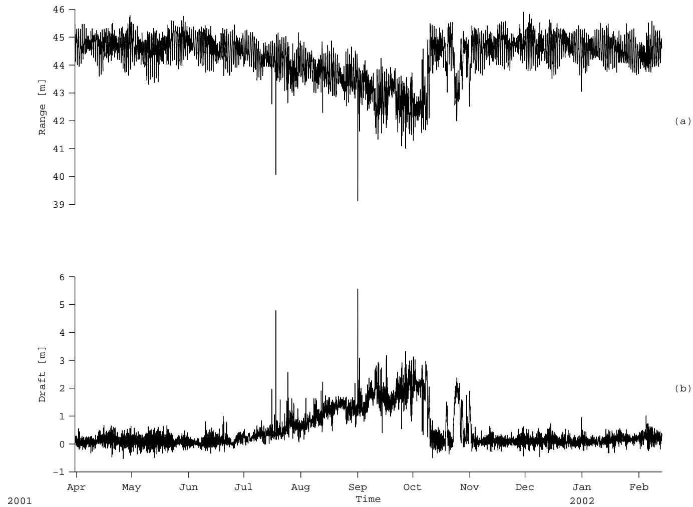
Figure 37: A2: Ice Profiler range (top panel) and draft (bottom panel)
