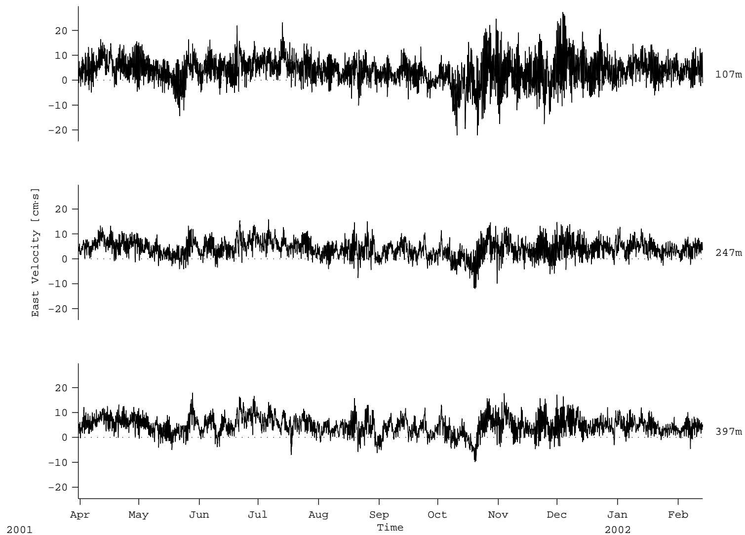
Figure 35: A2: VACM Velocity (East)
