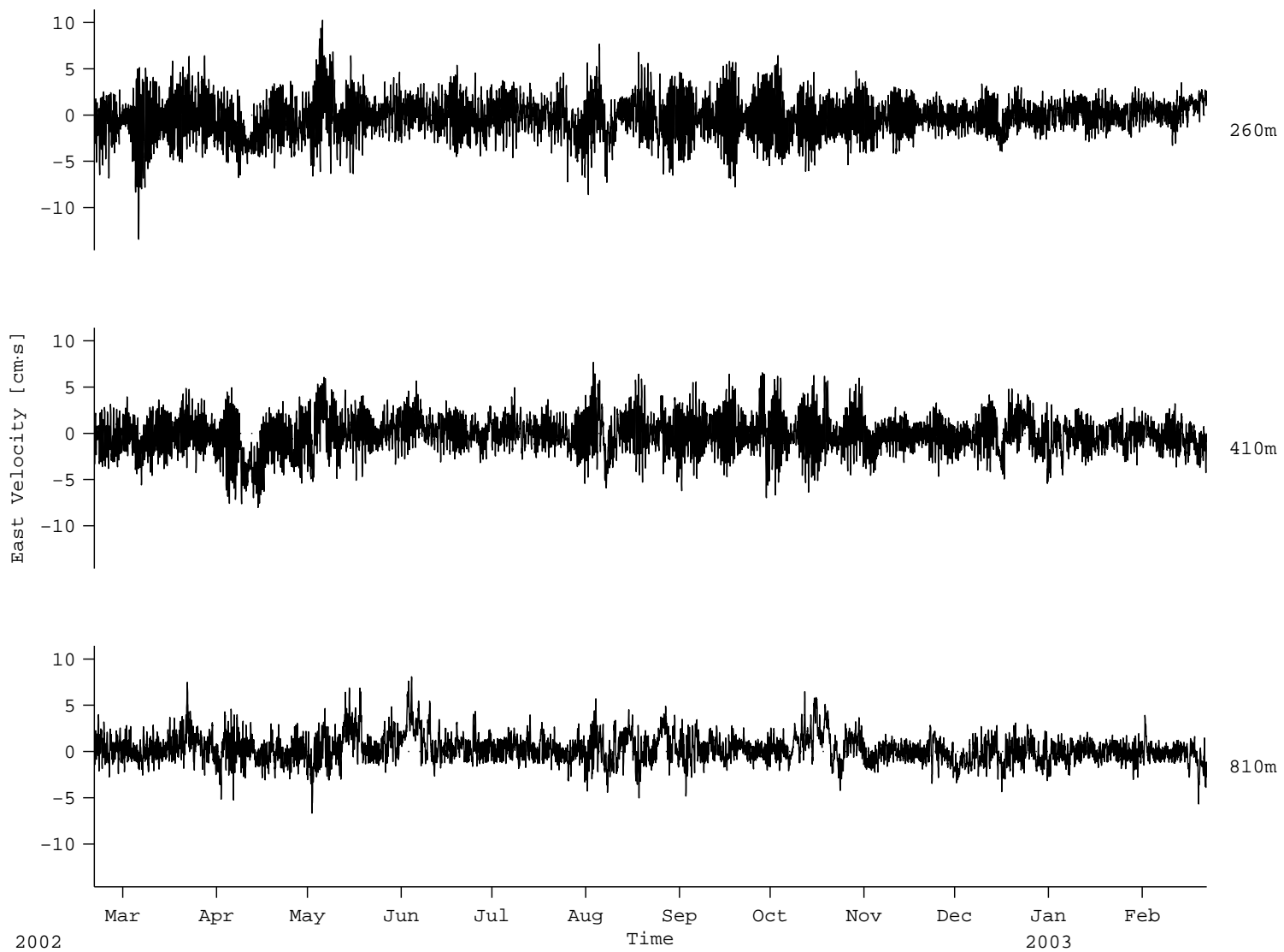
Figure 64: C2: VACM Velocity (East)
