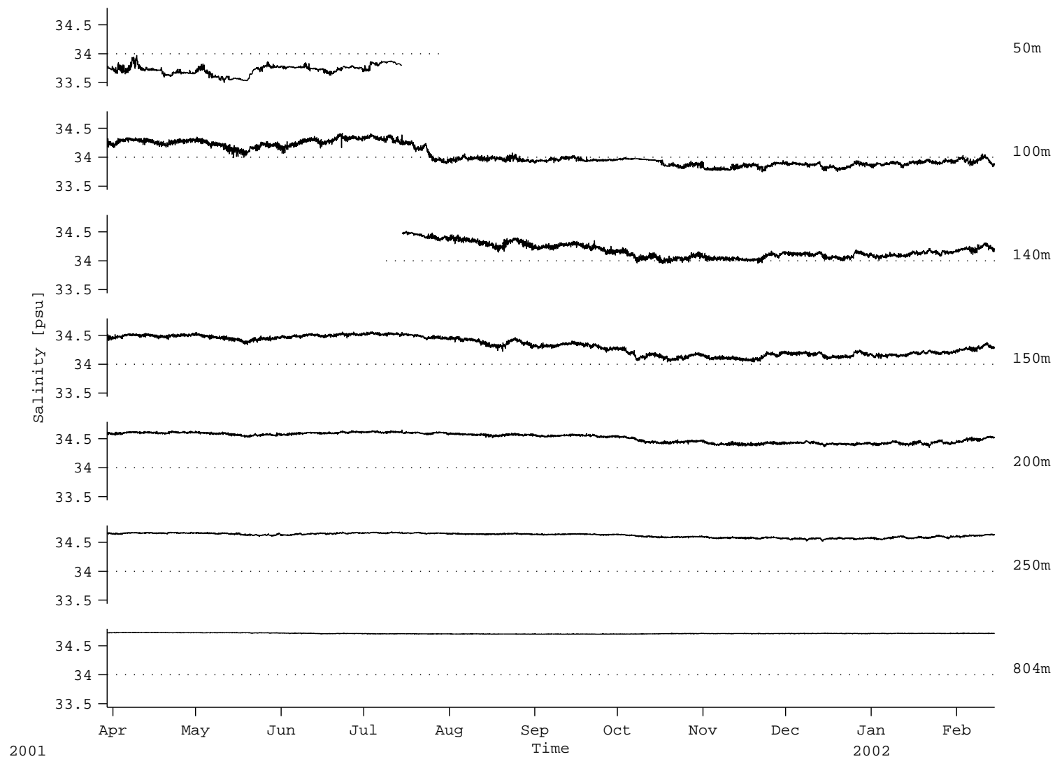
Figure 44: B2: Salinity records
