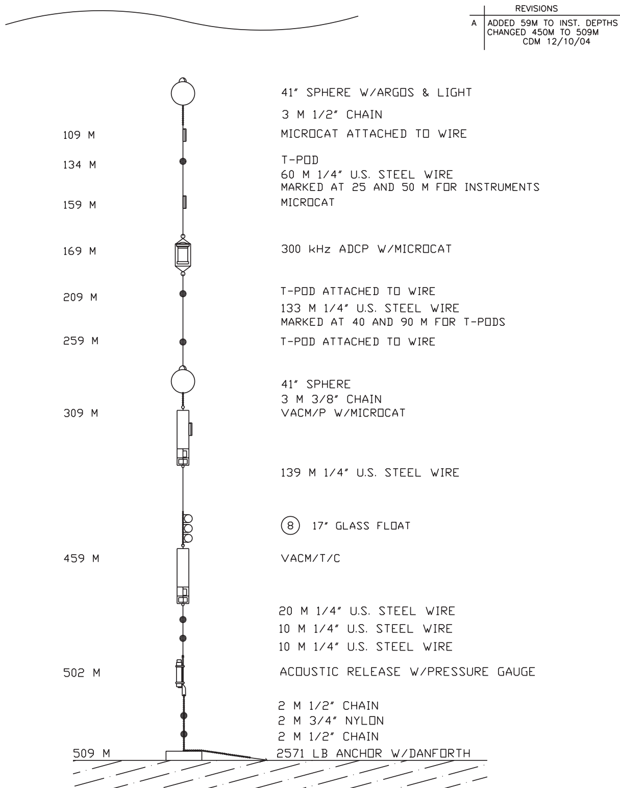
Figure 5: A1: Mooring Design.
