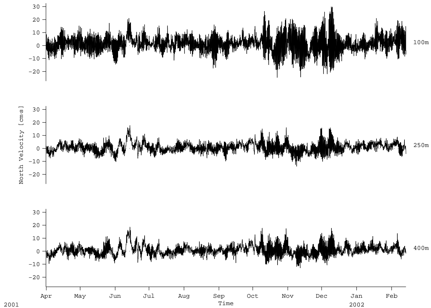
Figure 42: A3: VACM Velocity (North)
