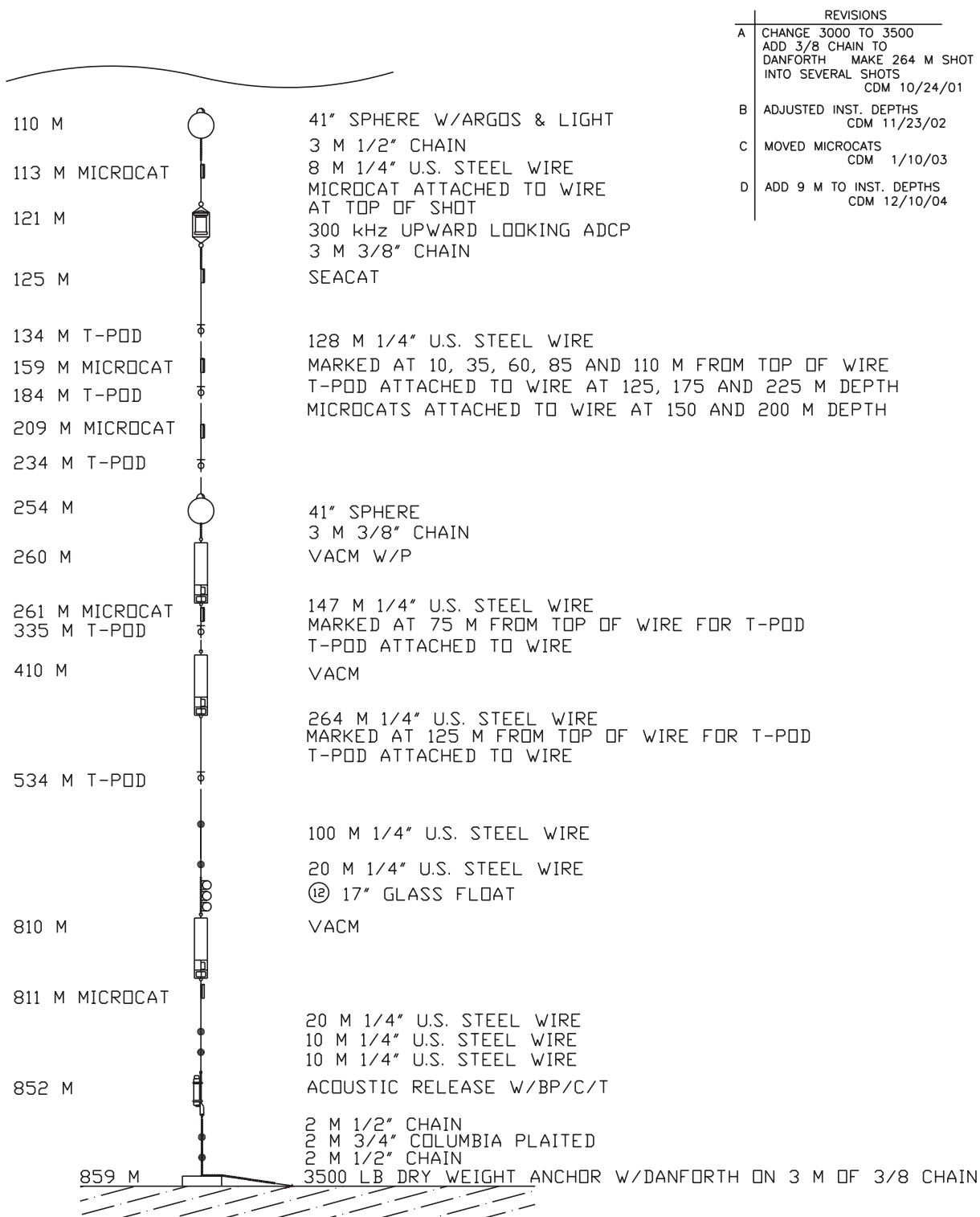
Figure 19: C2: Mooring Design.
