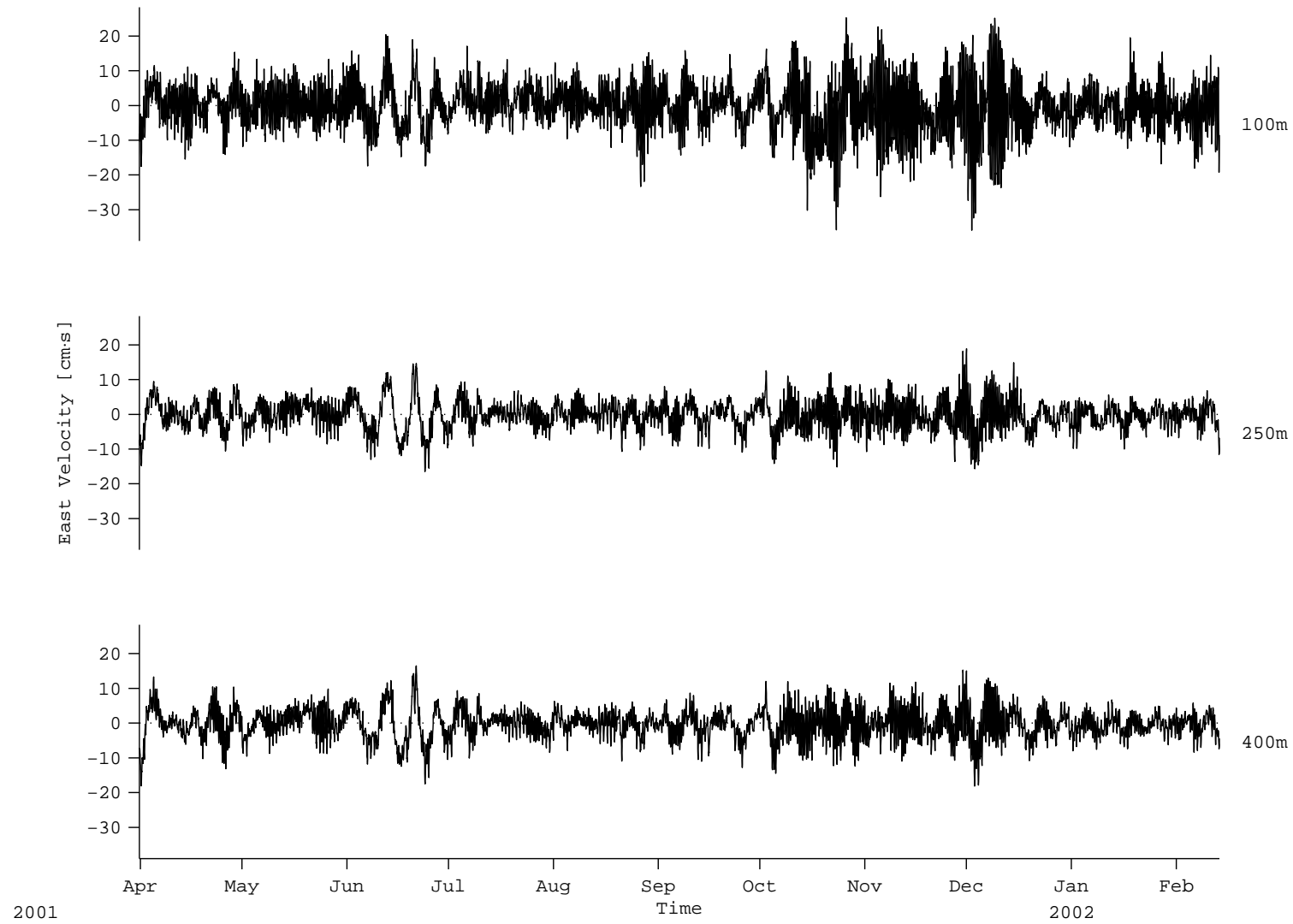
Figure 41: A3: VACM Velocity (East)
