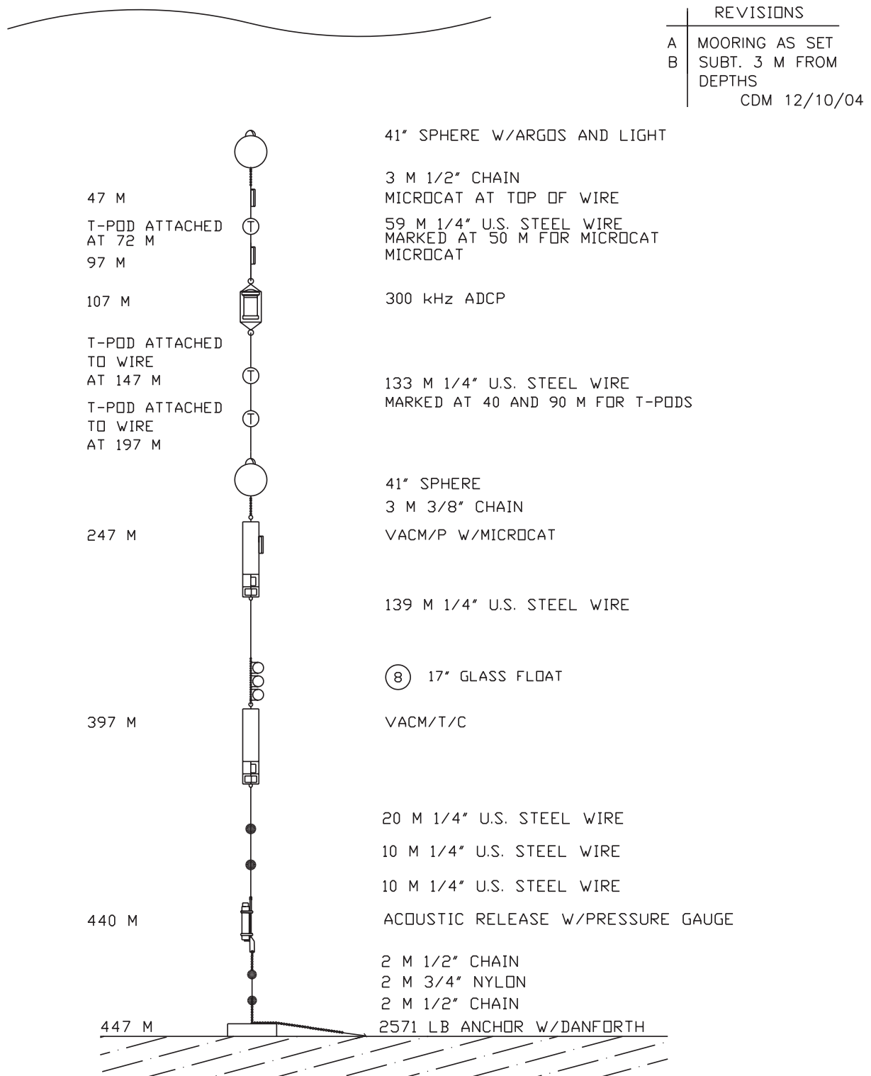
Figure 15: B3: Mooring Design.
