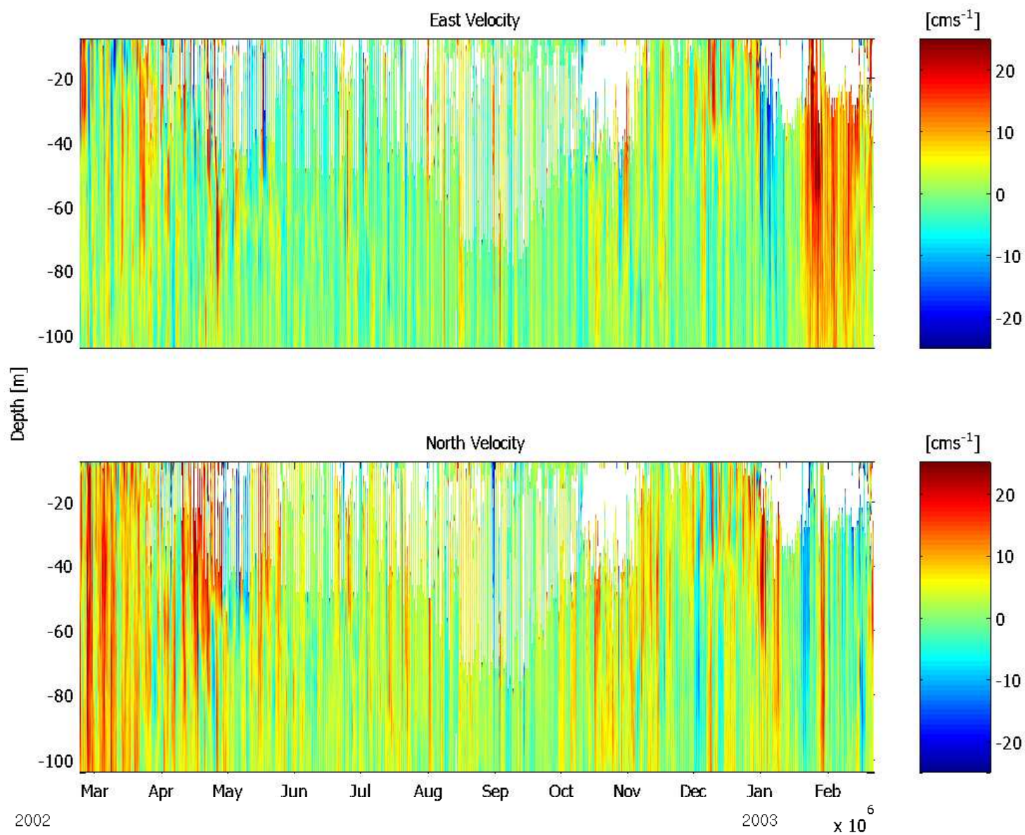
Figure 71: C3: ADCP Velocity. East Velocity (Top Panel), North Velocity (Bottom Panel)
