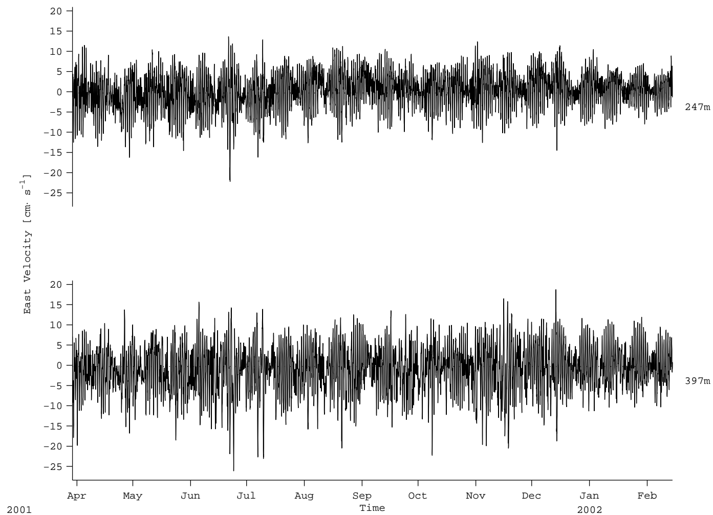
Figure 52: B3: VACM Velocity (East)
