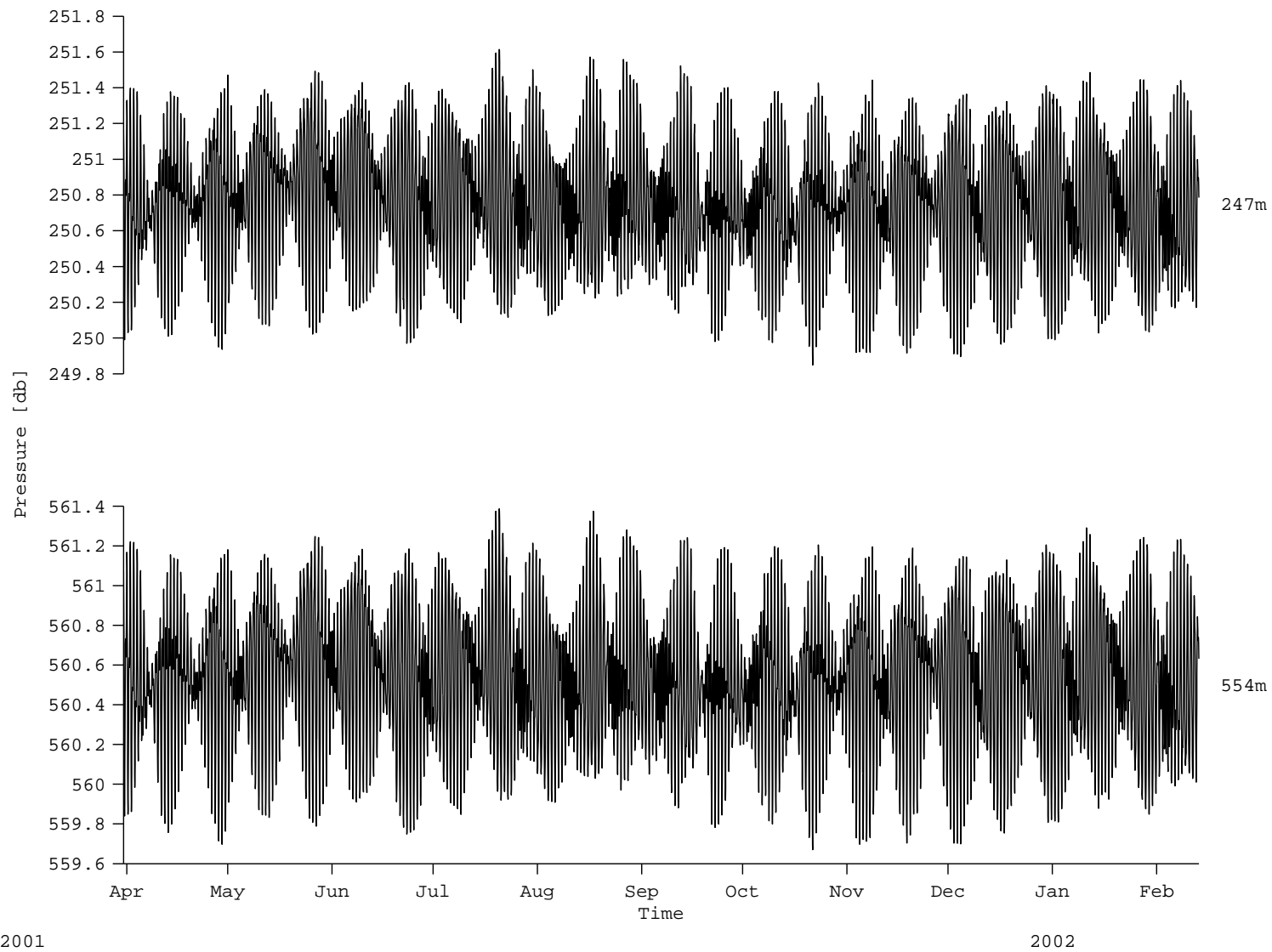
Figure 34: A2: Pressure records
