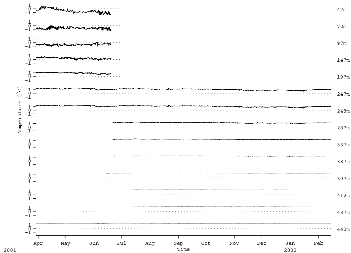
Figure 49: B3: Temperature records
