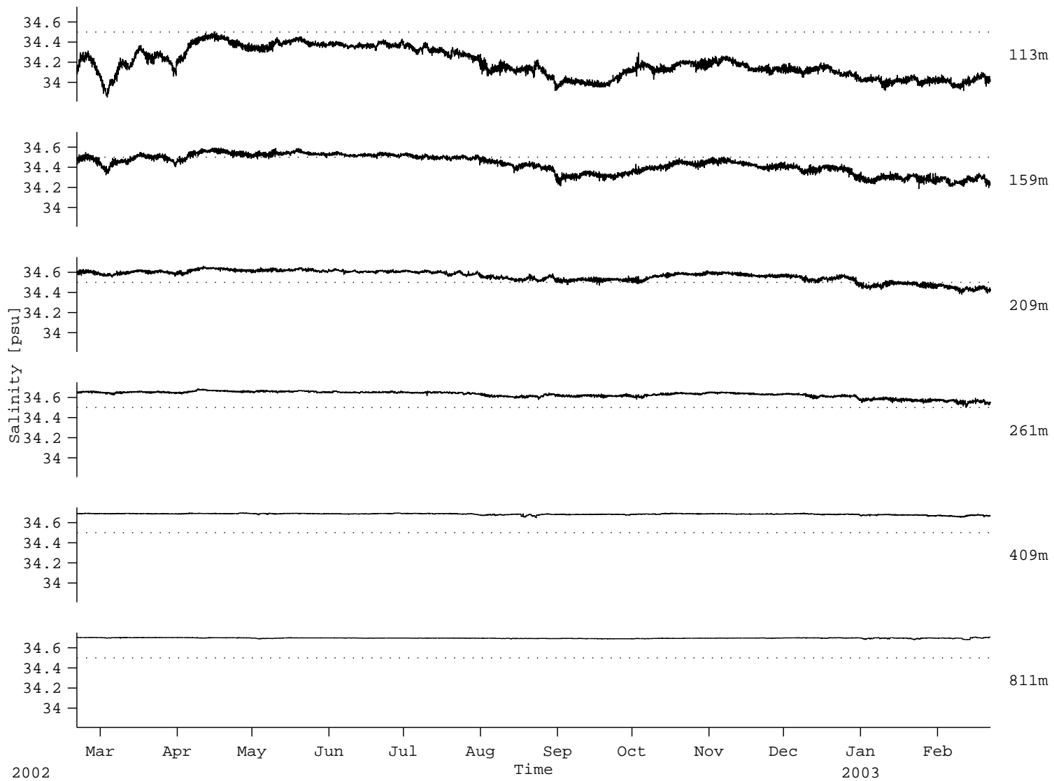
Figure 62: C2: Salinity records
