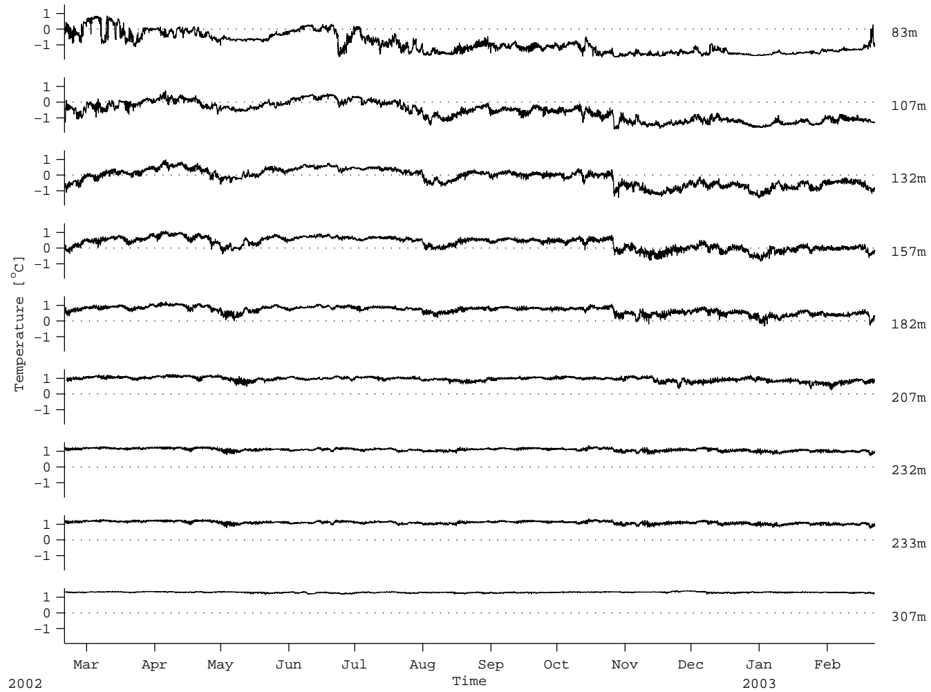
Figure 56: C1: Temperature records
