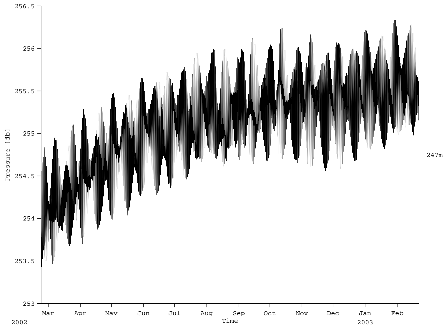
Figure 68: C3: Pressure records
