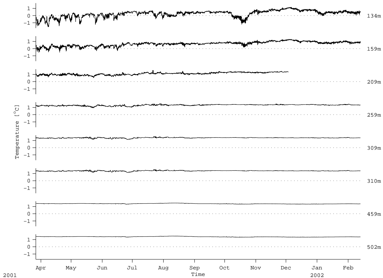
Figure 26: A1: Temperature records
