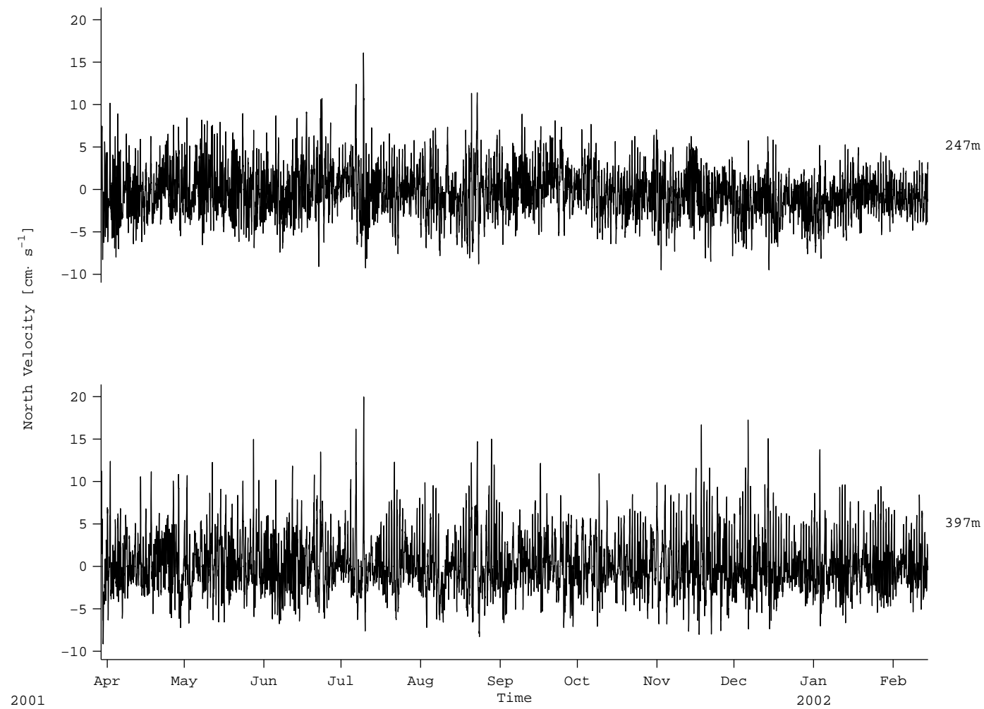
Figure 53: B3: VACM Velocity (North)
