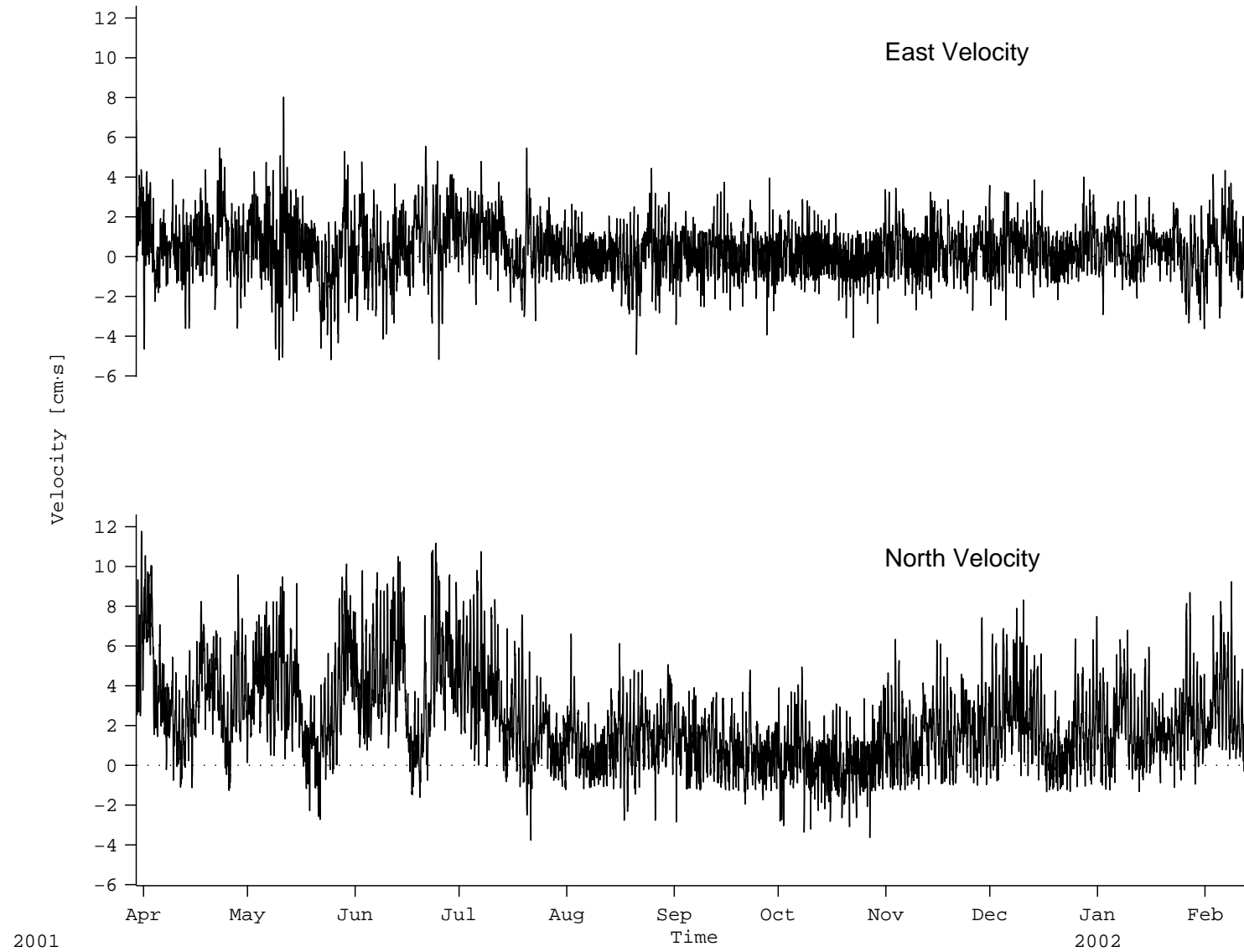
Figure 46: B2: VACM Velocity
