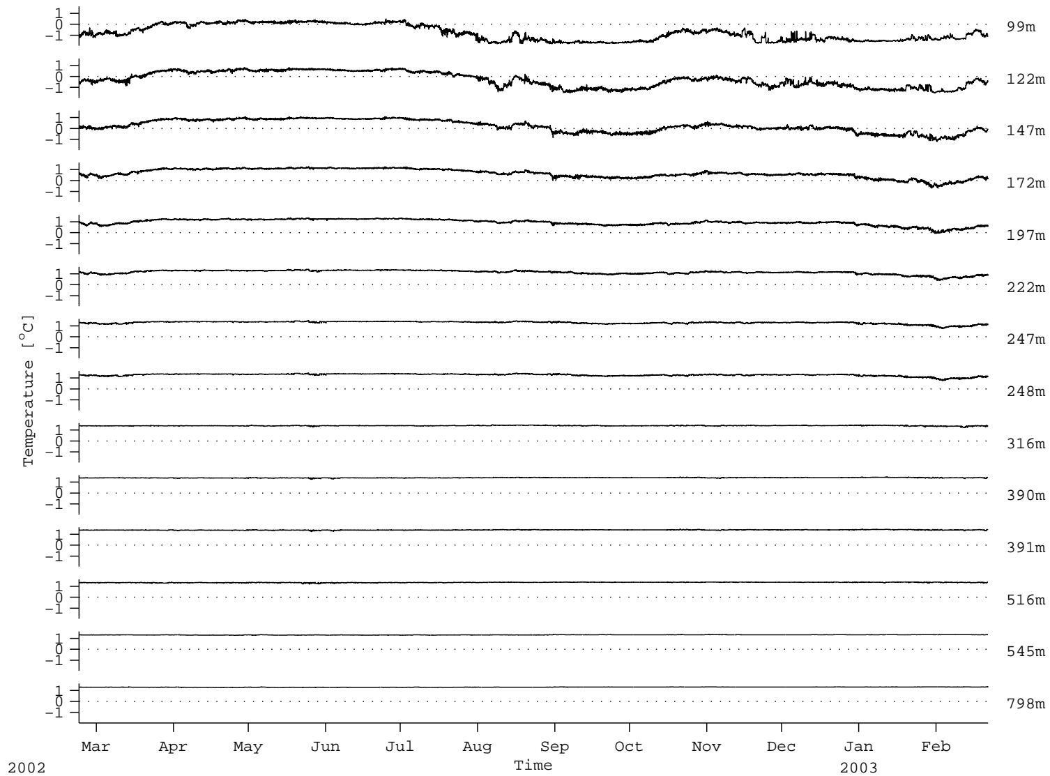
Figure 66: C3: Temperature records
