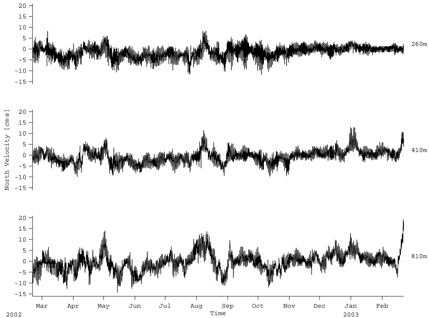
Figure 65: C2: VACM Velocity (North)
