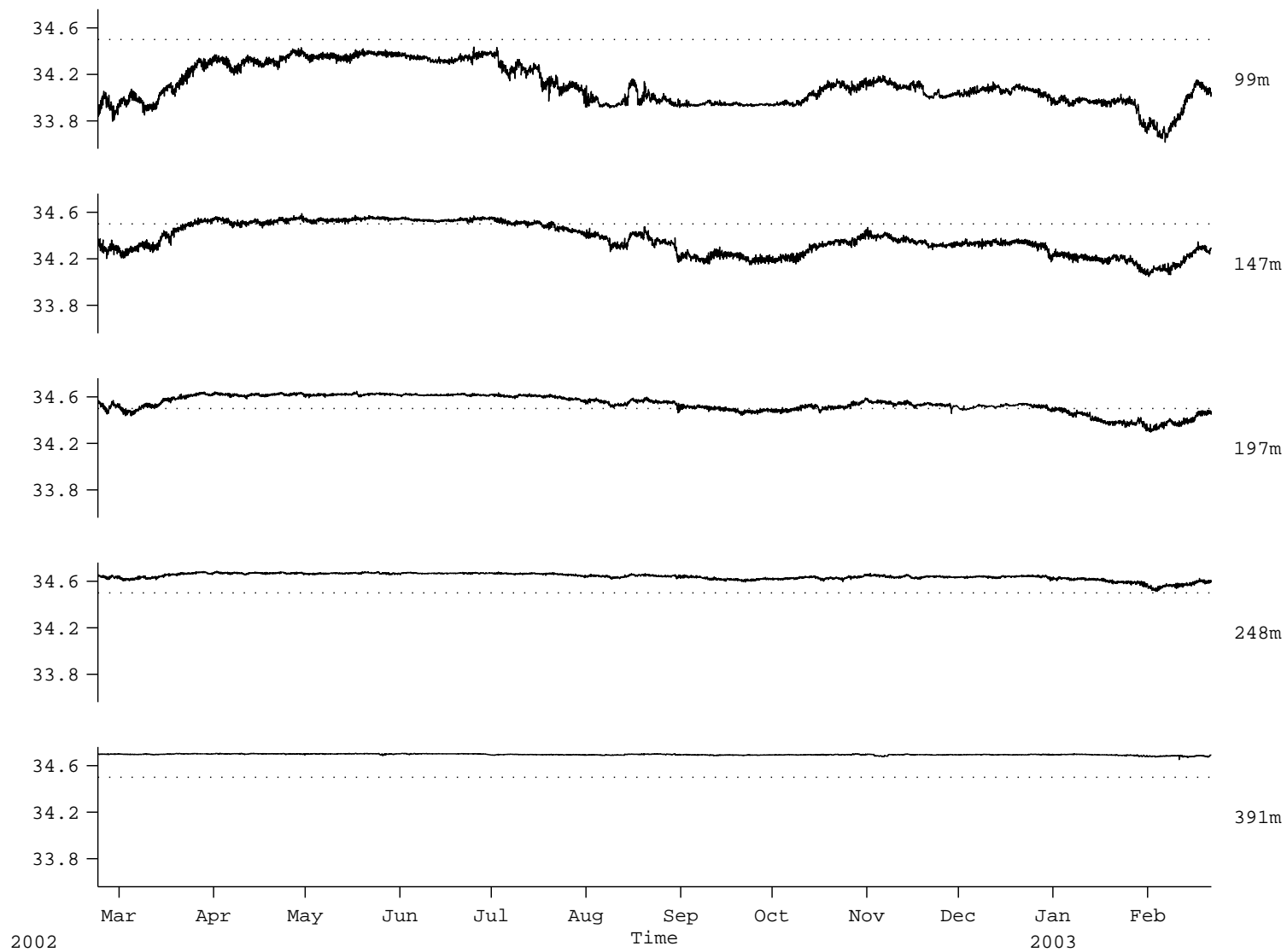
Figure 67: C3: Salinity records
