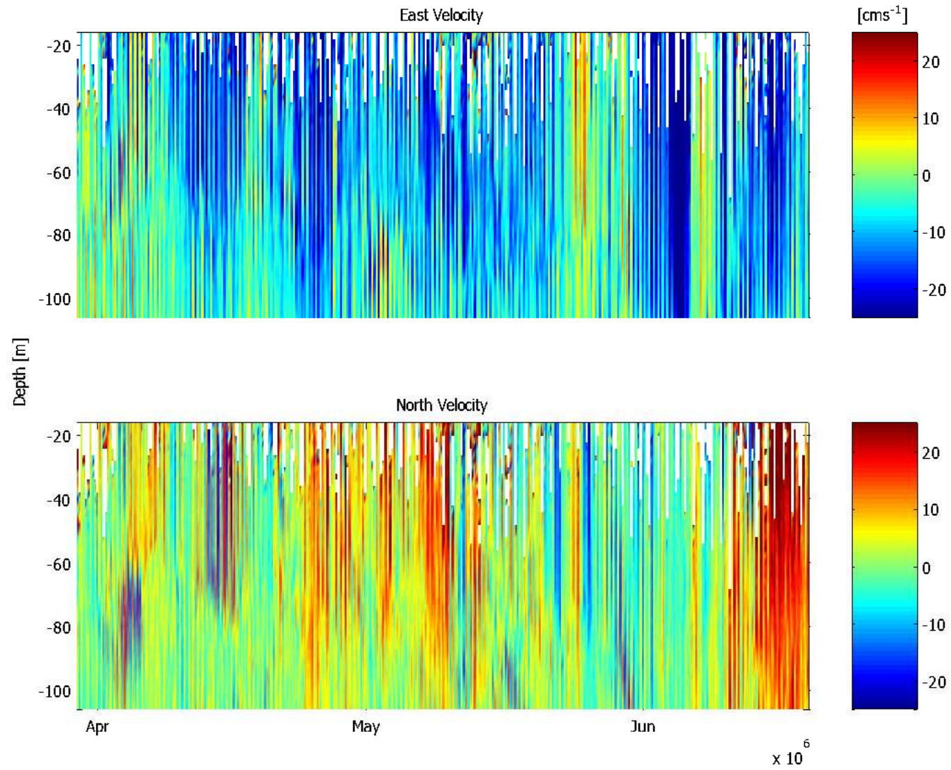
Figure 54: B3: ADCP Velocities, 110m
