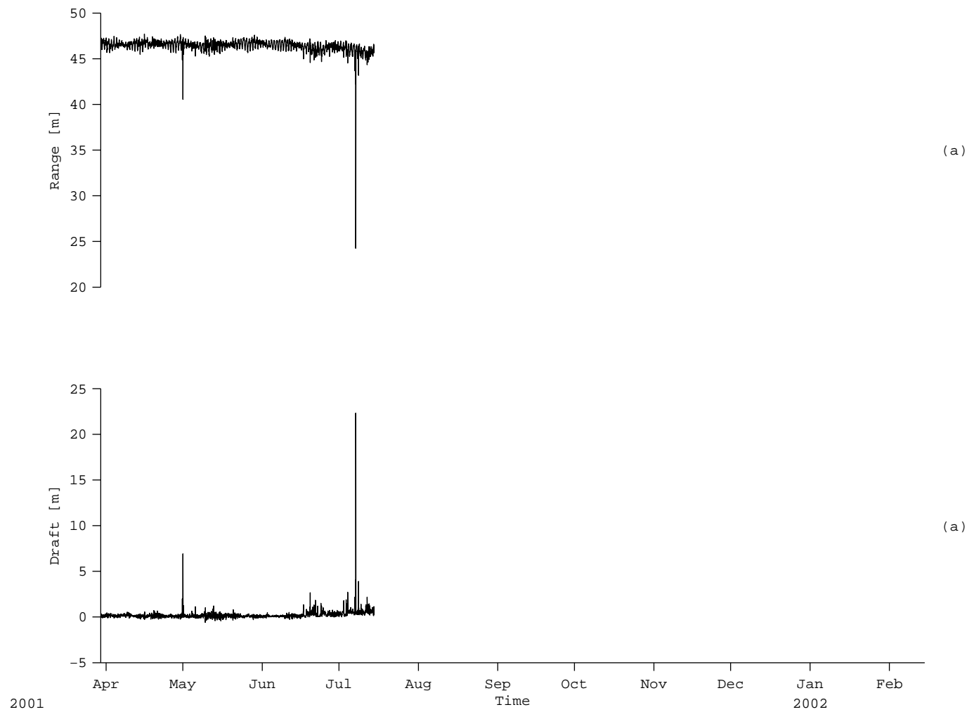
Figure 48: B2: Ice Profiler range (top panel) and draft (bottom panel)
