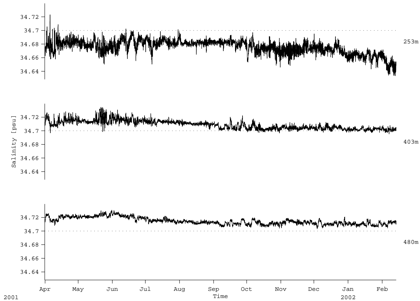
Figure 39: A3: Salinity records
