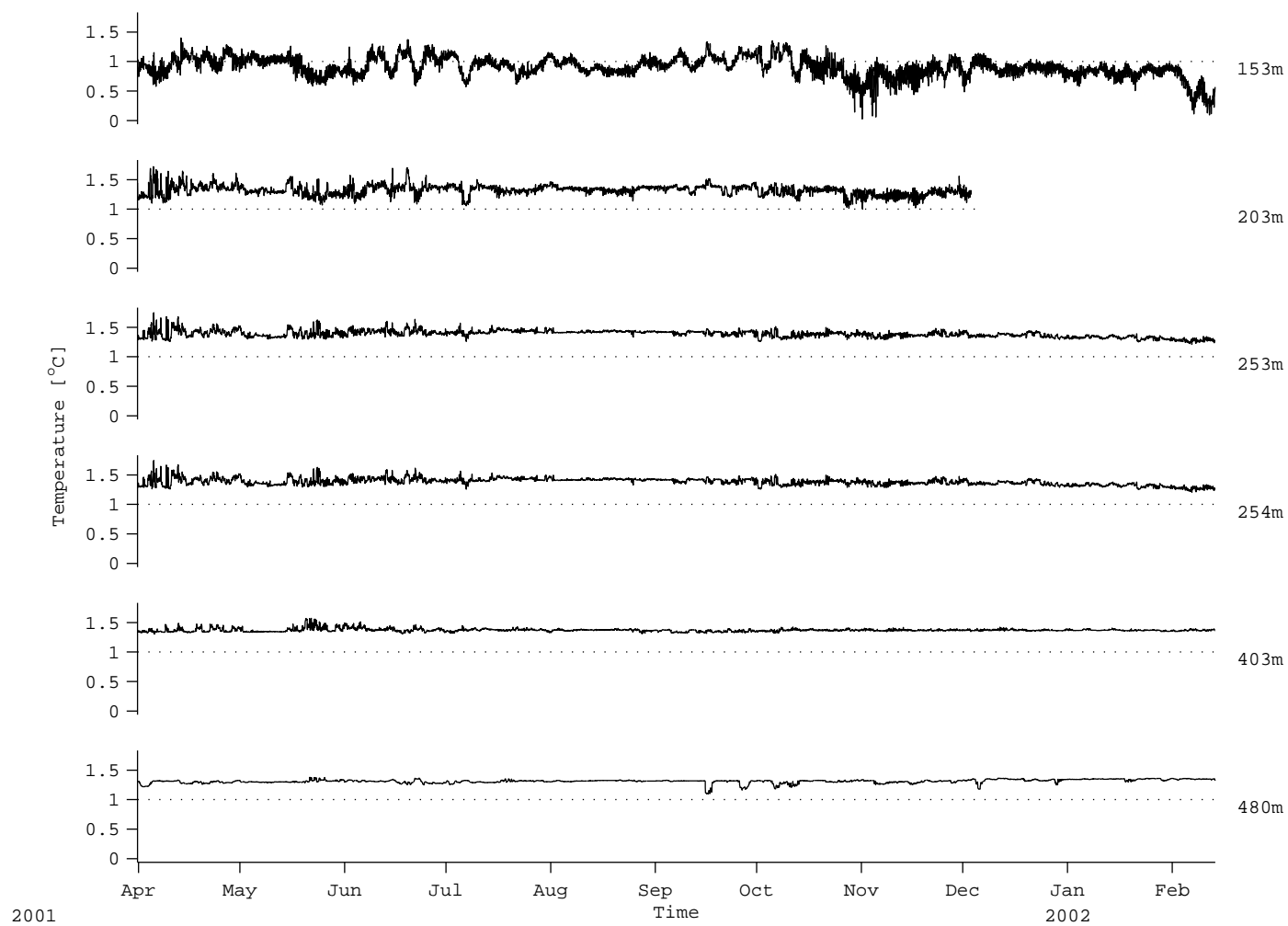
Figure 38: A3: Temperature records
