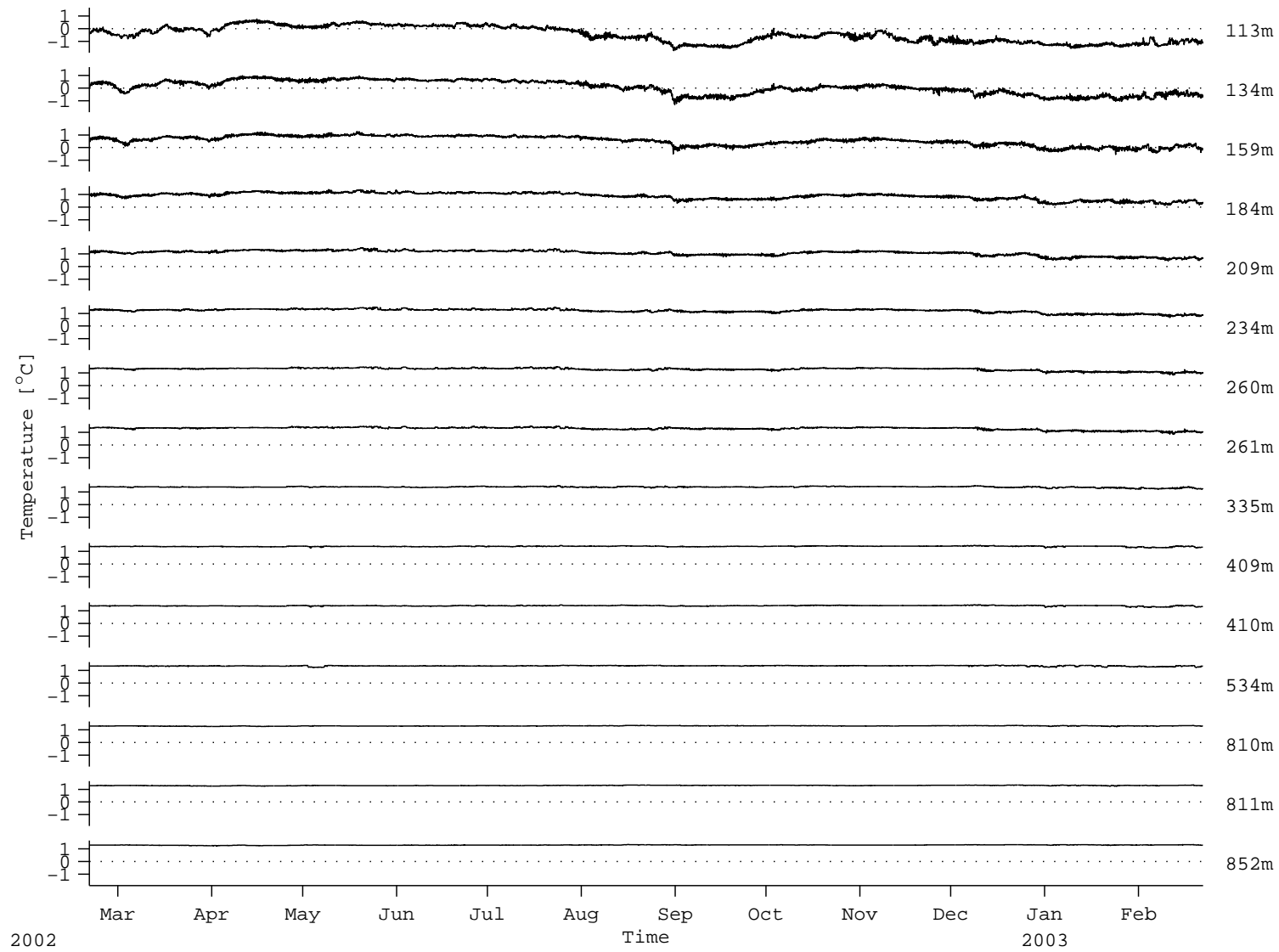
Figure 61: C2: Temperature records
