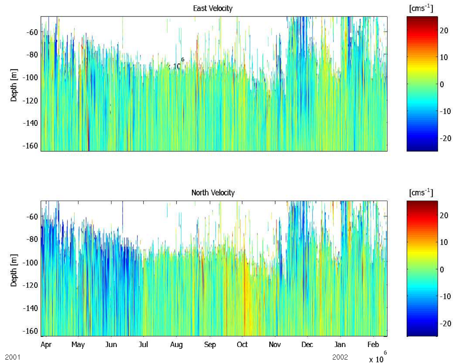
Figure 31: A1: ADCP Velocities
