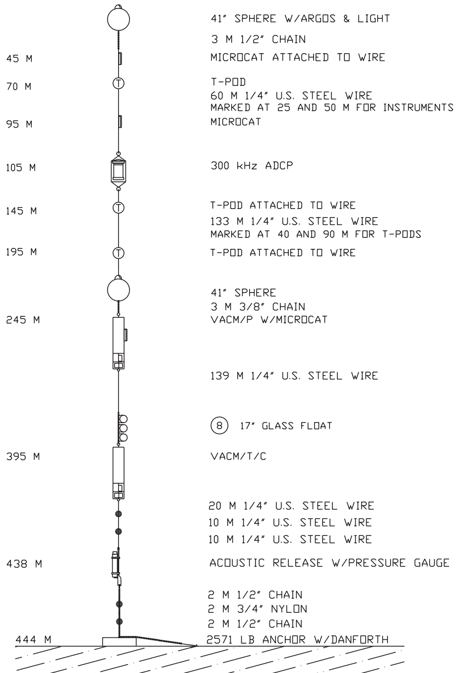
Figure 11: B1: Mooring Design.
