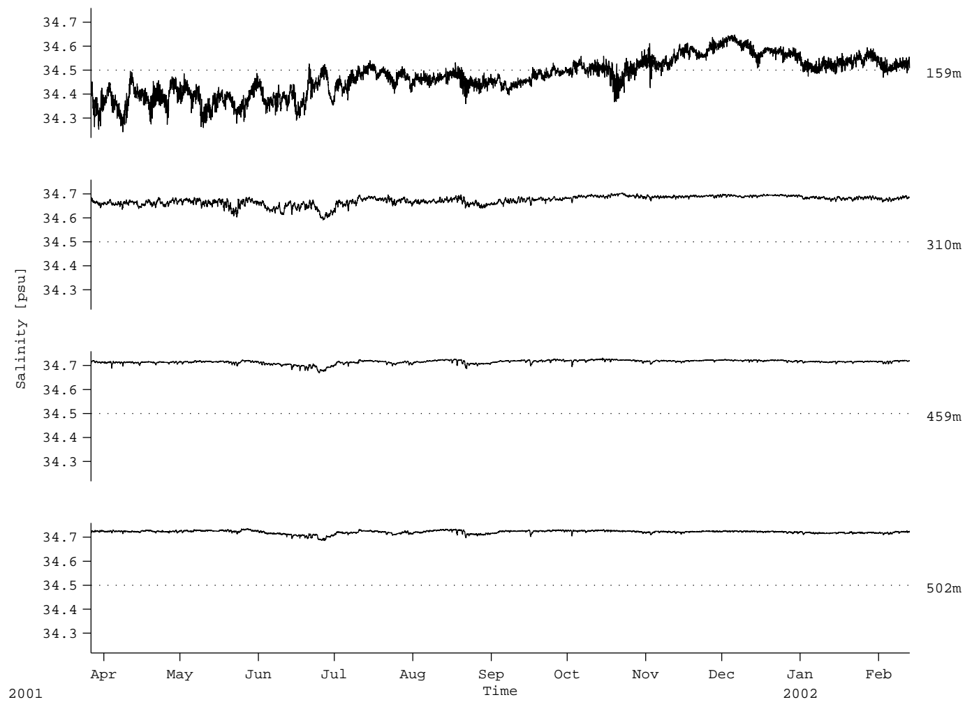
Figure 27: A1: Salinity records
