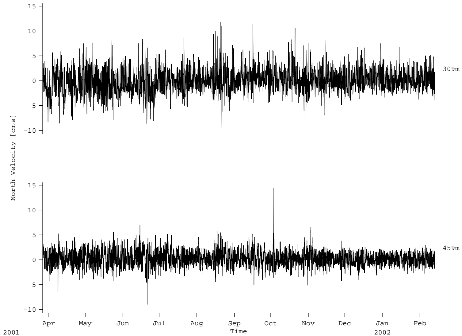
Figure 30: A1: VACM Velocities (North)
