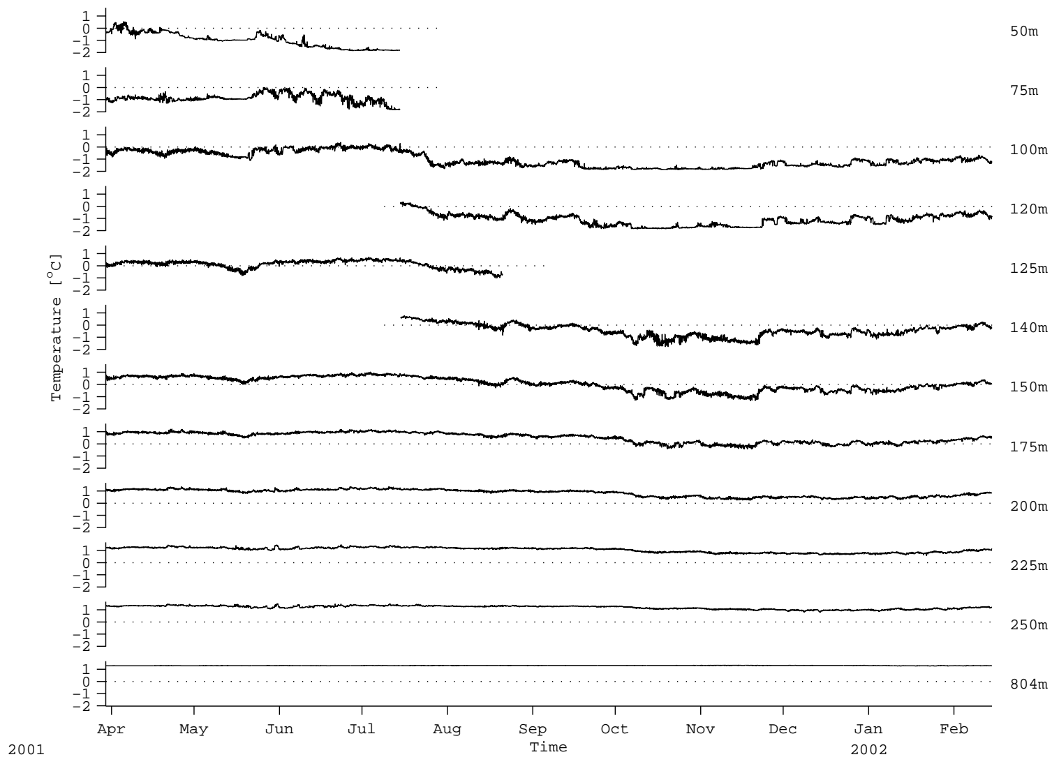
Figure 43: B2: Temperature records
