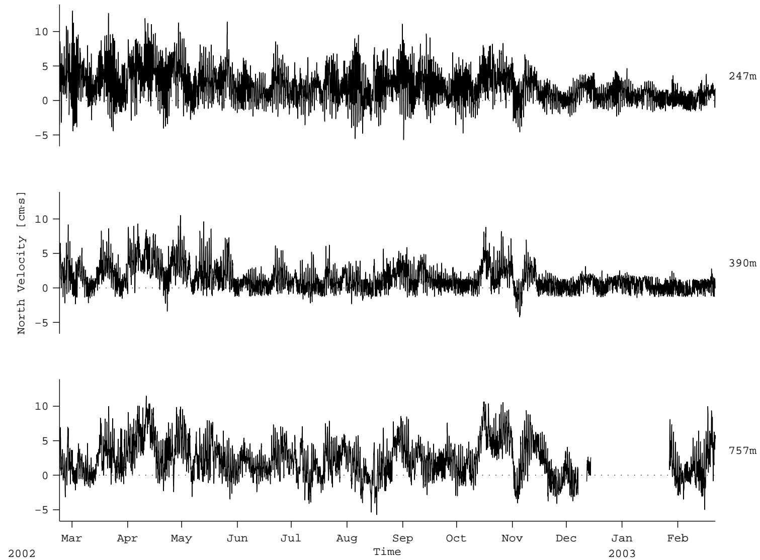
Figure 70: C3: VACM Velocity (North)
