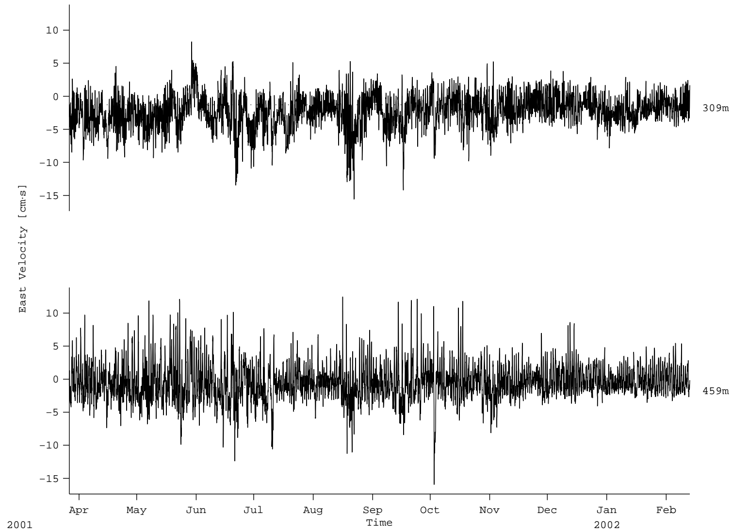
Figure 29: A1: VACM Velocities (East)
