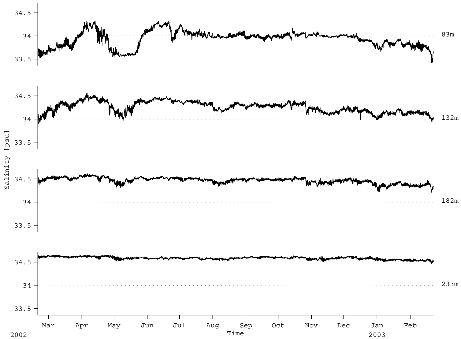
Figure 57: C1: Salinity records
