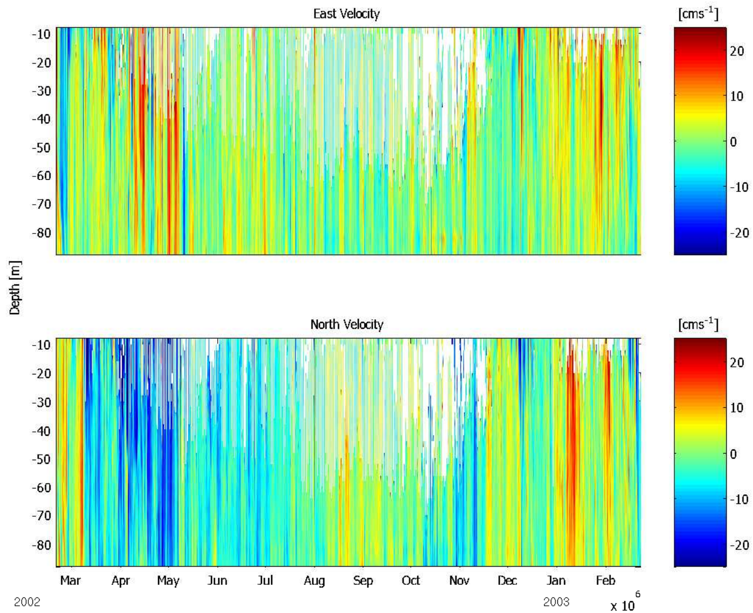
Figure 60: C1: ADCP Velocities
