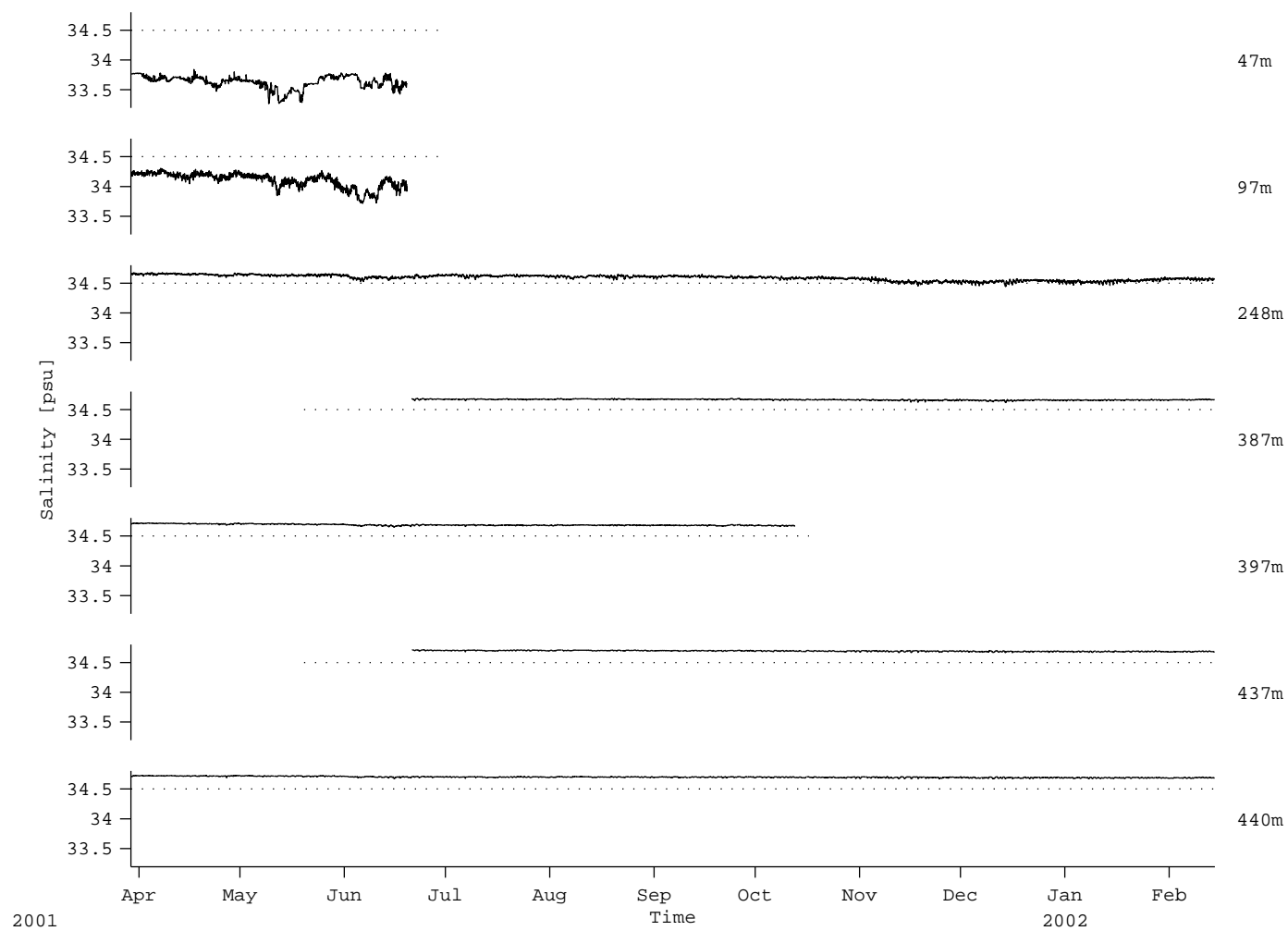
Figure 50: B3: Salinity records
