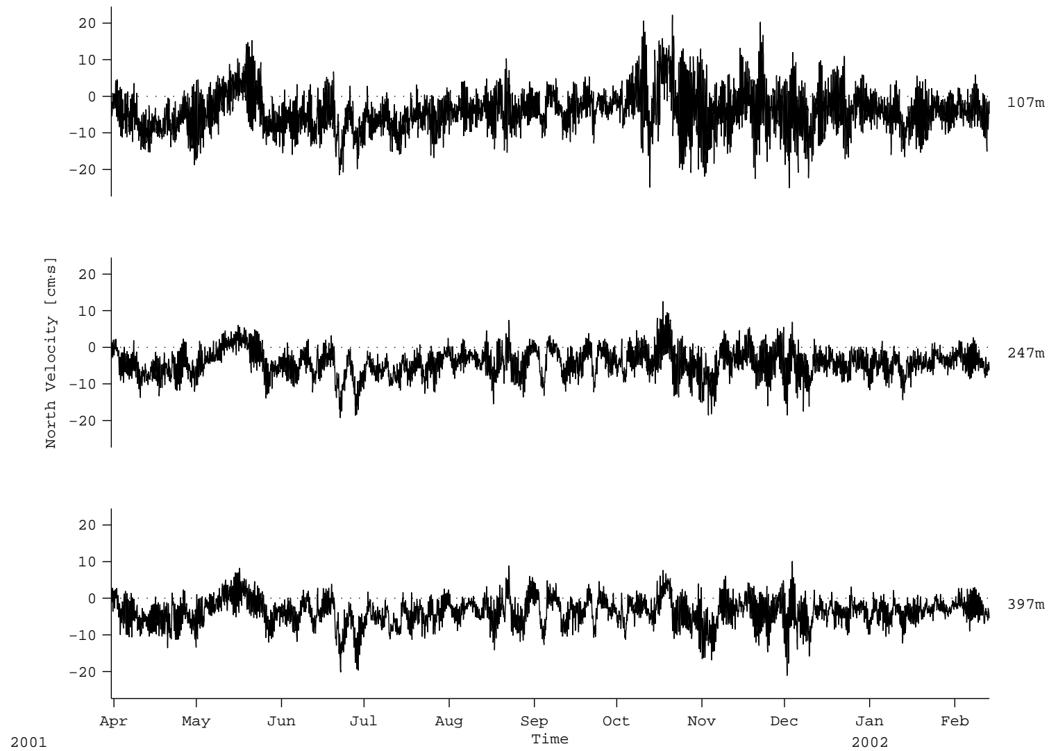
Figure 36: A2: VACM Velocity (North)
