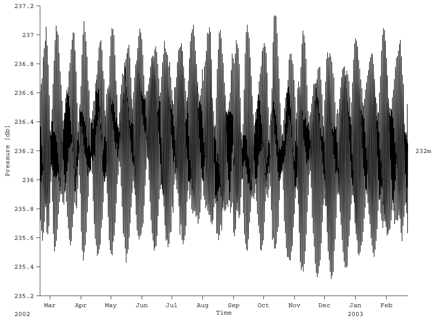
Figure 58: C1: Pressure records
