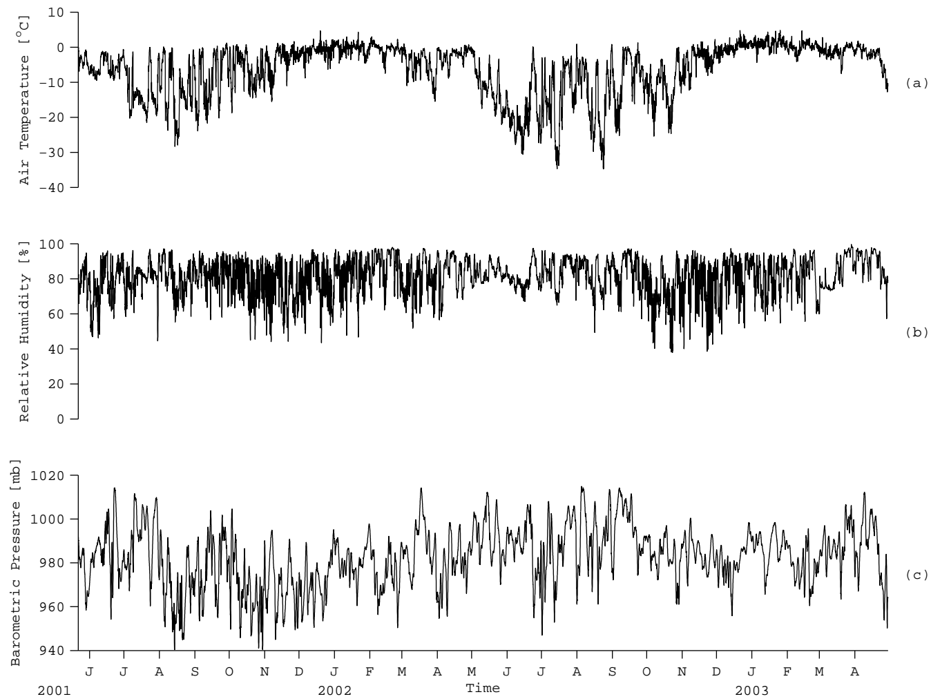
Figure 75: Air temperature (a), relative humidity (b) and barometric pressure (c) measured with the AWS at Kirkwood Island
