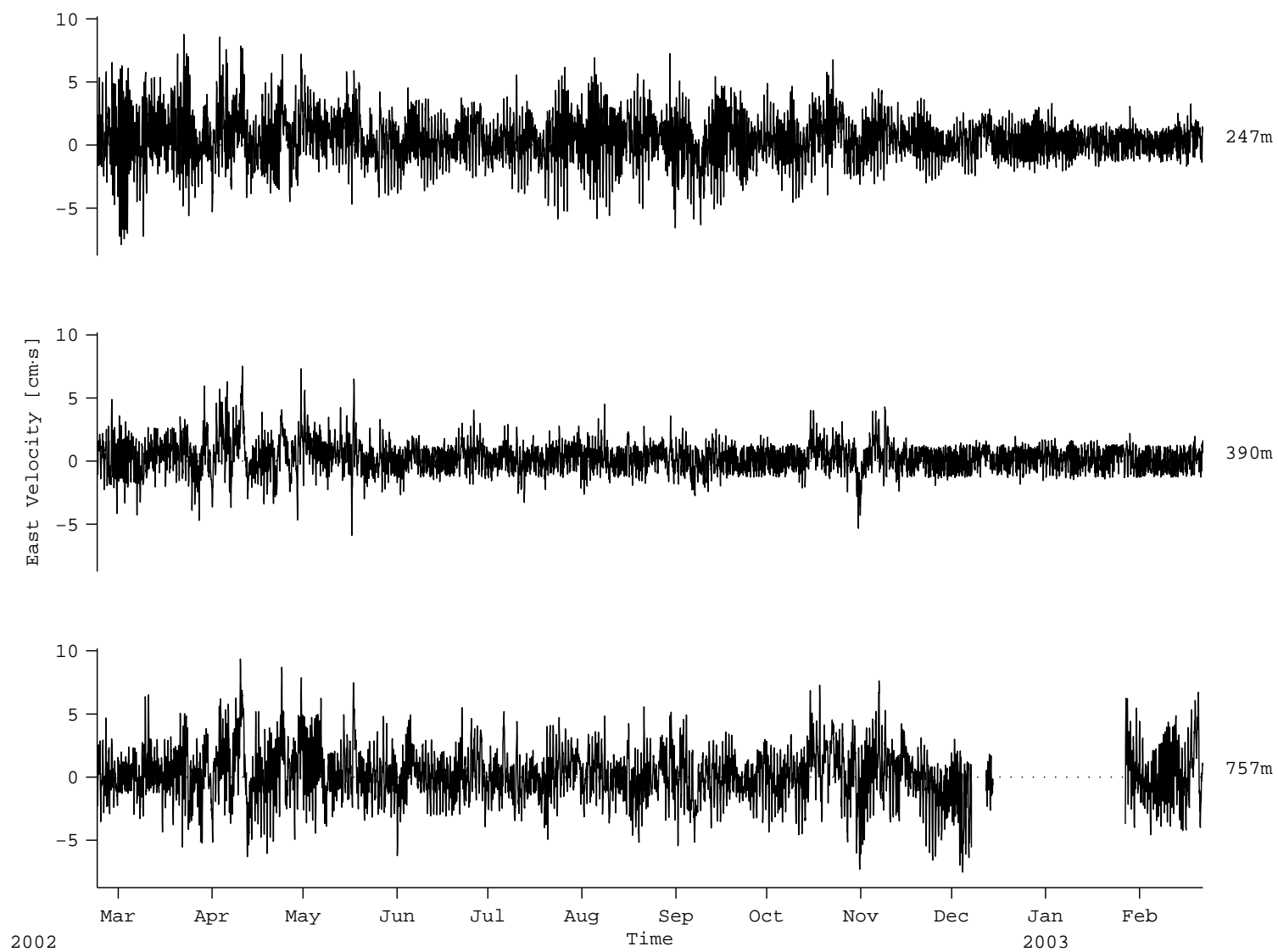
Figure 69: C3: VACM Velocity (East)
