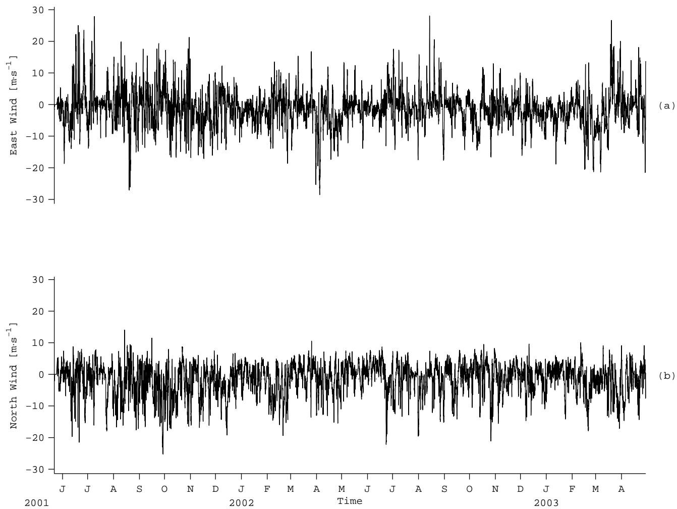
Figure 74: Wind speed in the East (a) and North (b) directions measured with the AWS at Kirkwood Island
