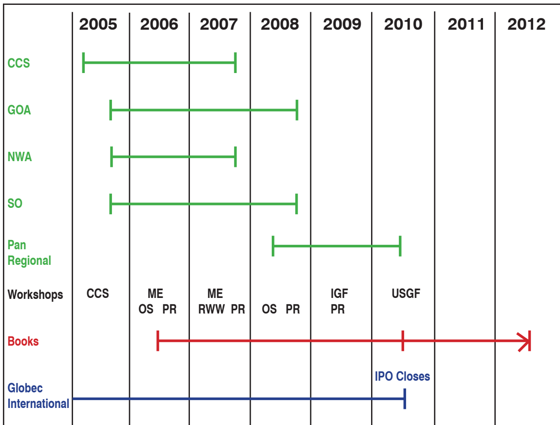
Figure 7. Proposed timeline for workshops, and special sessions to facilitate GLOBEC synthesis. IGF: International GLOBEC Final Symposium; ME: Model Evaluation Workshop, OS: Ocean Sciences; PR: Pan Regional Workshop; RWW: Regional (GB, SO, NEP) Workshops; USGF: U.S. GLOBEC Final Symposium.
