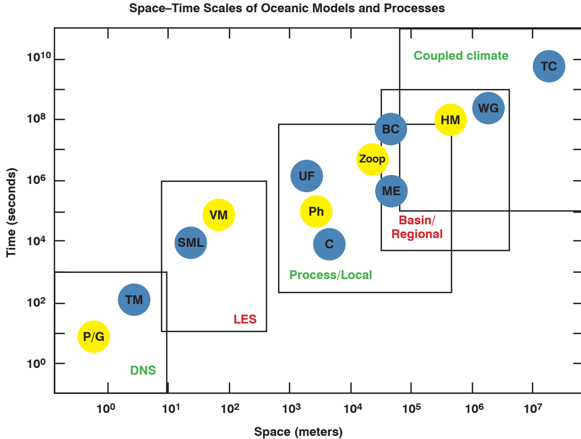
Figure 3. Space-time diagram showing some physical and biological processes of interest to the U.S. GLOBEC program. Physical processes are shown in blue, and include: turbulent mixing (TM), surface mixed layer processes (SML), upwelling fronts (UF), convection (C), boundary currents (BC), mesoscale eddies (ME), the North Atlantic Oscillation (NAO), El Niño-Southern Oscillation (ENSO) and the Pacific Decadal Oscillation (PDO). Biological processes (in yellow) are: predation/grazing (P/G), vertical migration (VM), horizontal migration (HM), and the natural scales of aggregation for phytoplankton (Ph) and zooplankton (Zoop). The rectangular boxes in green and red show the approximate space/time scales covered by five classes of ocean and/or ocean/atmosphere models: Coupled climate, Basin/regional, Process-oriented /Local, Large-eddy simulation (LES) and Direct numerical simulation (DNS). [from Mantua et al. 2002]
