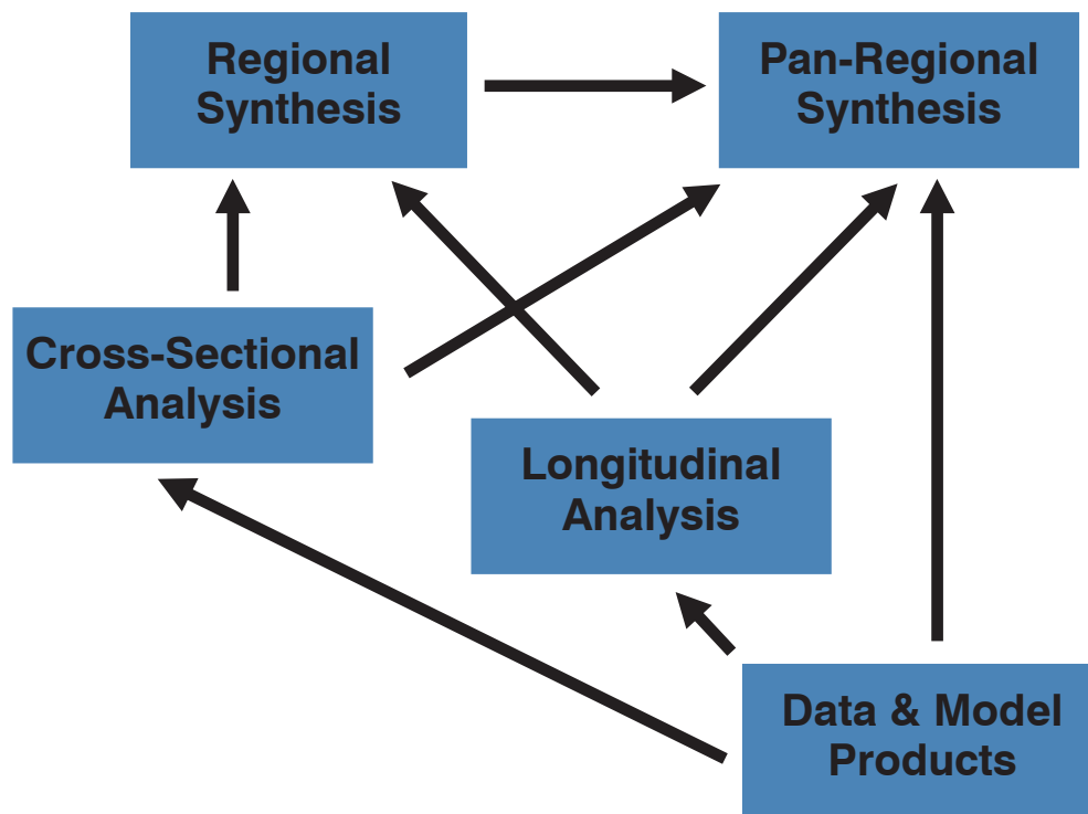
Figure 1. Options for comparative analysis within and among GLOBEC studies to achieve Regional and Pan-regional synthesis using a combination of longitudinal and cross-sectional analyses.
