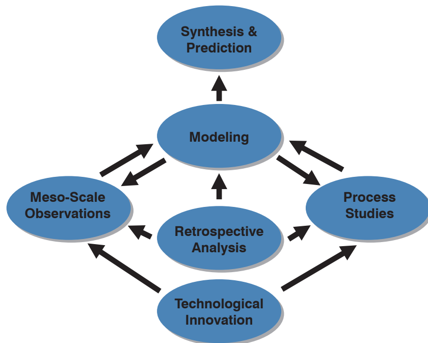
Figure 2. Key elements of the GLOBEC research strategy, culminating in synthesis
