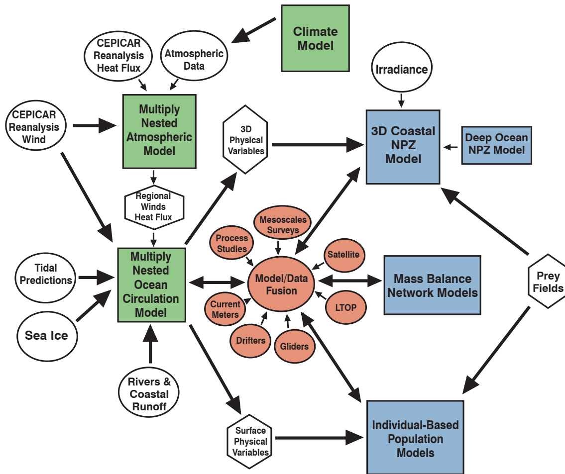
Figure 4. Schematic diagram of one possible configuration for a multi-scale GLOBEC model of the future based on the nesting concept. The primary elements of the modeling system include (1) a climate forcing model (2) a nested hierarchy of (global/basin/regional/local) physical circulation models for the ocean and atmosphere (3) one or more food web models including mass balance network models and NPZ models (4) one or more individual-based models for the relevant higher trophic level species and finally (5) appropriate mechanisms (possibly utilizing advanced data assimilation) for comparison and/or fusion of these forward models with the available retrospective and contemporary data sets (modified from Mantua et al. 2002).
